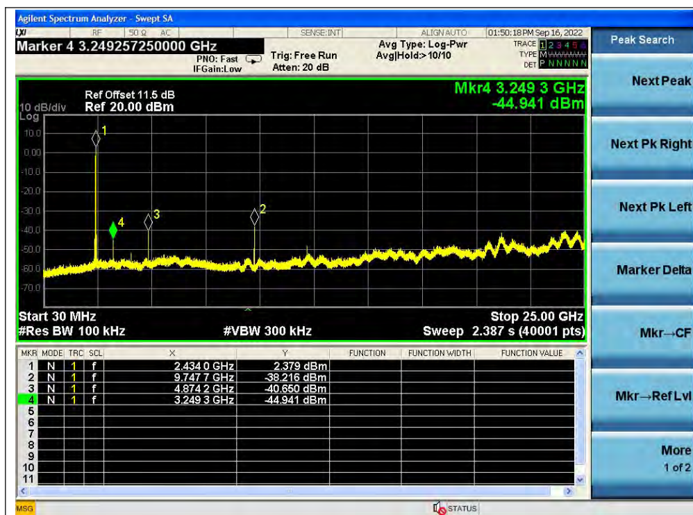
(30MHz to 25GHz, Channel 6, 802.11b)
