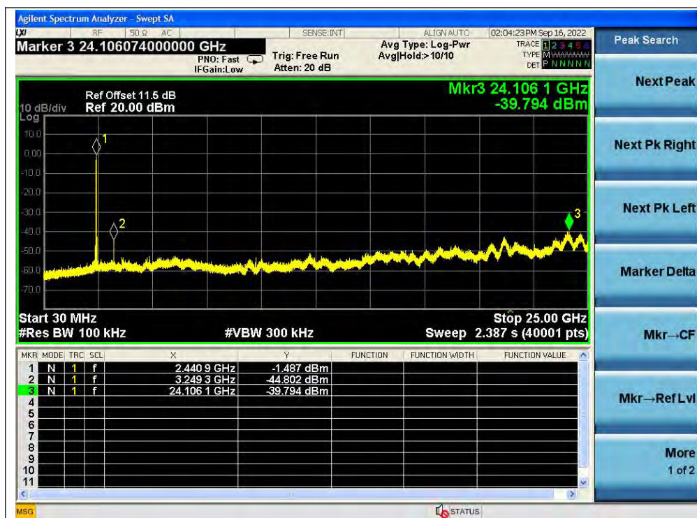
(30MHz to 25GHz, Channel 6, 802.11n (HT20))
