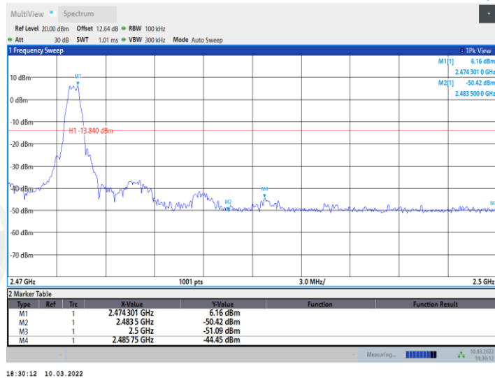
Ant1_High_2474
