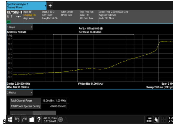
B2_N30(10M)_DFT-s- OFDM_BPSK_Edge_1RB_Left_Low_CH_CHP_PAS
