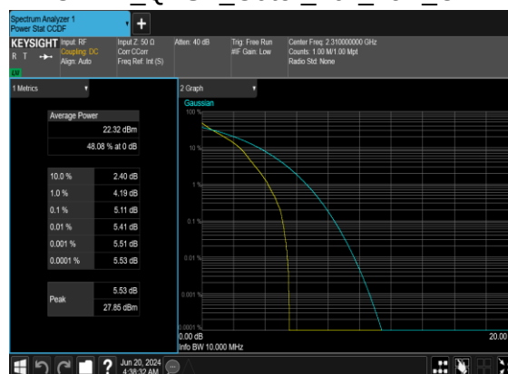
B2_N30(10M)_DFT-s- OFDM QPSK Outer Full Low CH
