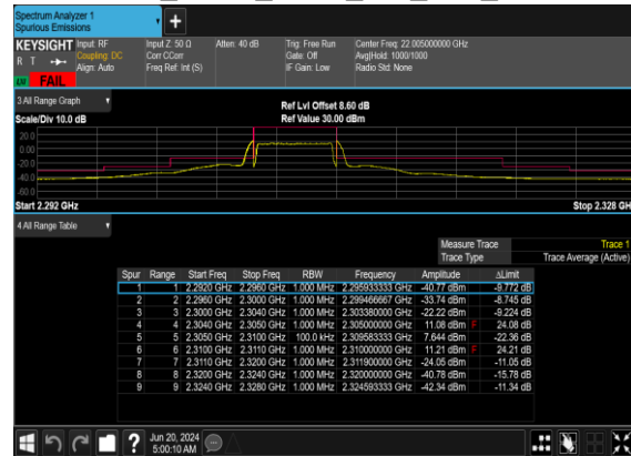
B2_N30(5M)_DFT-s- OFDM_BPSK_Outer_Full_Low_CH
