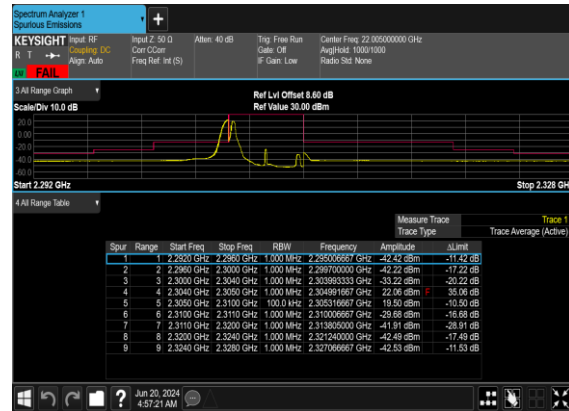
B2_N30(5M)_DFT-s- OFDM_QPSK_Edge_1RB_Left_Low_CH
