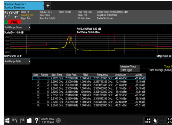
B2_N30(10M)_DFT-s- OFDM_QPSK_Edge_1RB_Left_Low_CH
