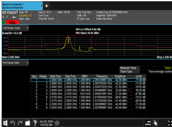
B2_N30(5M)_DFT-s- OFDM_BPSK_Edge_1RB_Left_Low_CH
