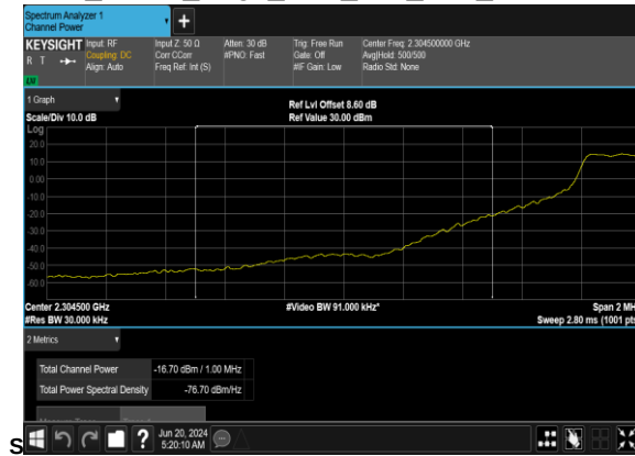
B2_N30(10M)_DFT-s- OFDM_QPSK_Edge_1RB_Left_Low_CH_CHP_PAS
