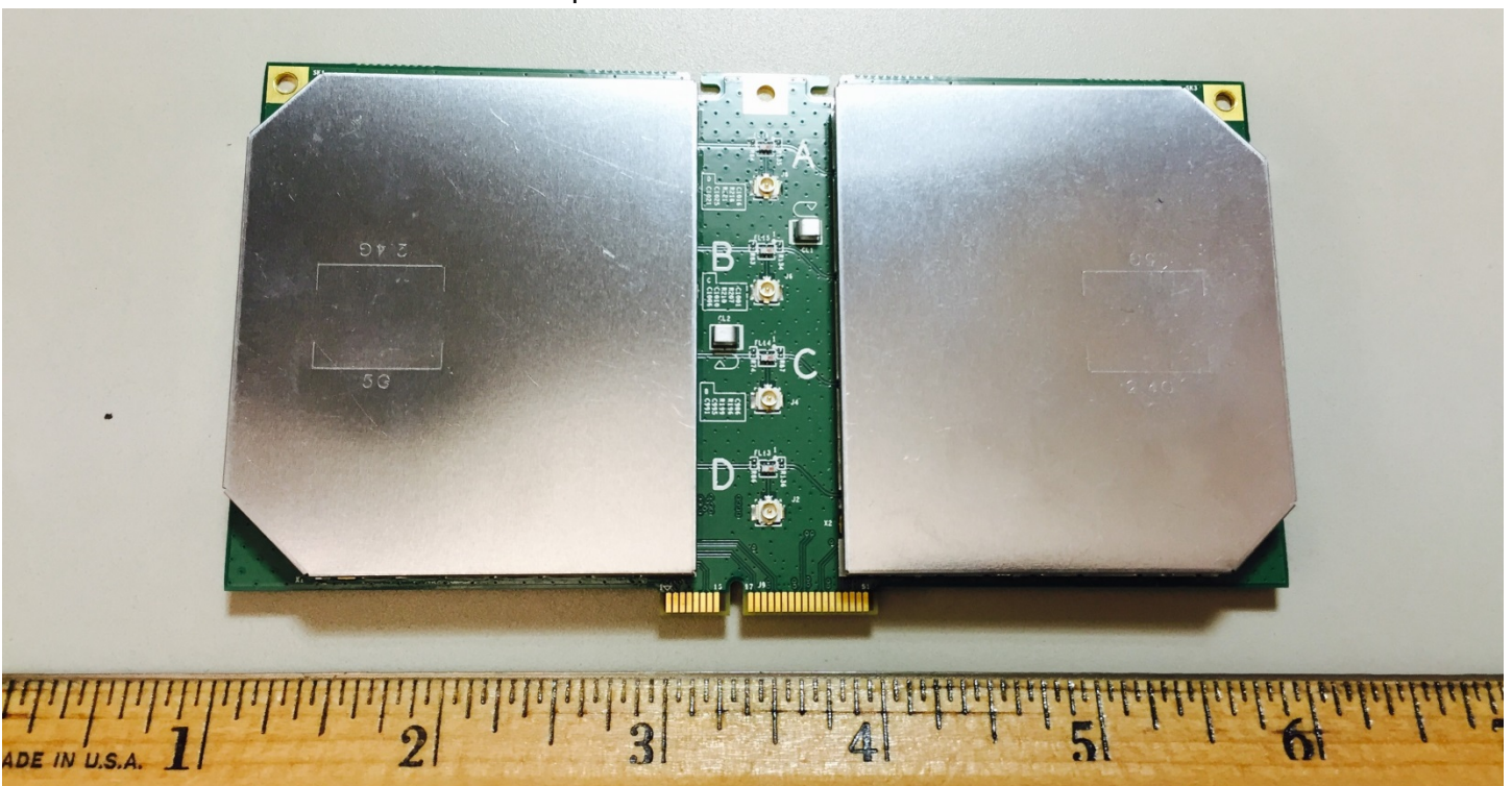
Top Side RF Board with Shields
