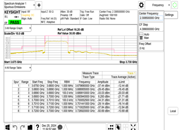
Emission Mask_Band48_10MHz_QPSK_RB50_0_CH56690
