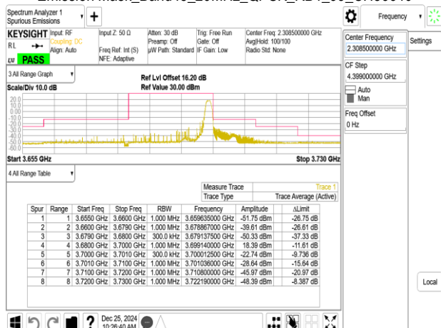
Emission Mask_Band48_20MHz_QPSK_RB1_99_CH56640
