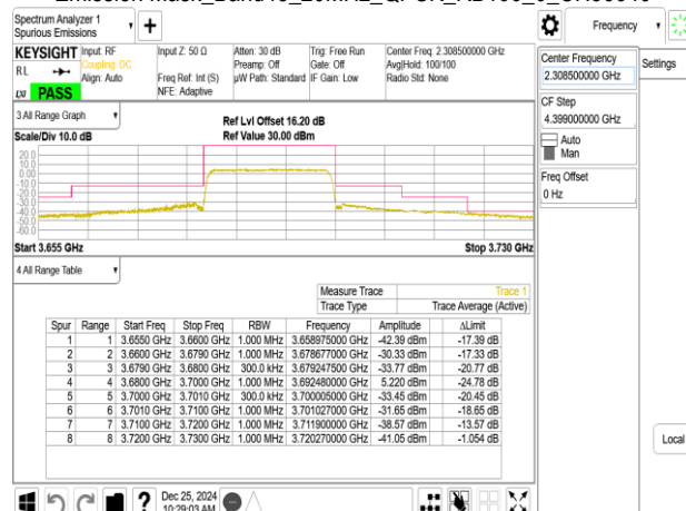
Emission Mask_Band48_20MHz_QPSK_RB100_0_CH56640
