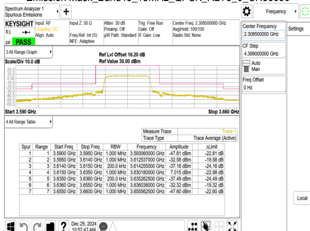
Emission Mask_Band48_15MHz_QPSK_RB75_0_CH56665
