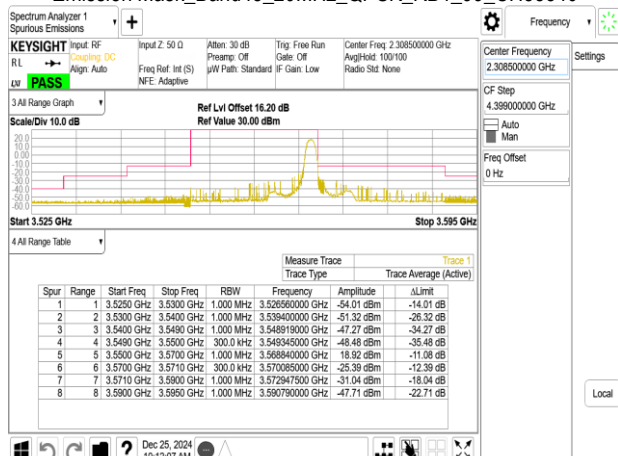
Emission Mask_Band48_20MHz_QPSK_RB1_99_CH55990
