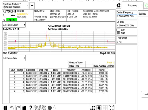
Emission Mask_Band48_20MHz_QPSK_RB1_0_CH56640
