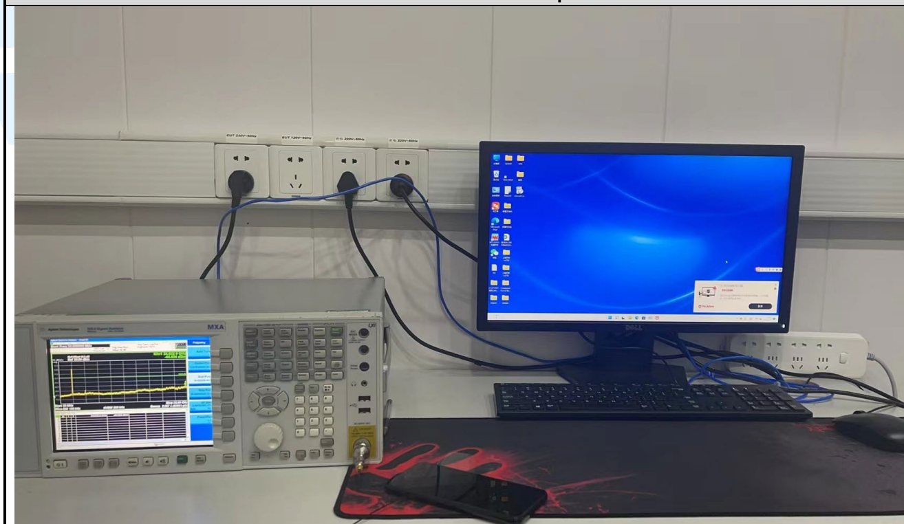
RF Conducted Test Setup
