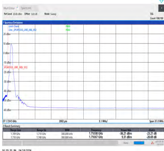
1-N66-15-30-L-4-CP-QPSK-Edge_1RB_Left-1@0-Ant1-1-seegraph-PASS-see graph
