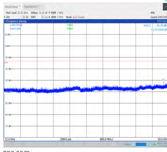
1-N66-15-40-L-1-DFT-PI2BPSK-Inner_1RB_Left-1@ 1-12000-20000-Ant1-19751.60--32.70--13-PASS
