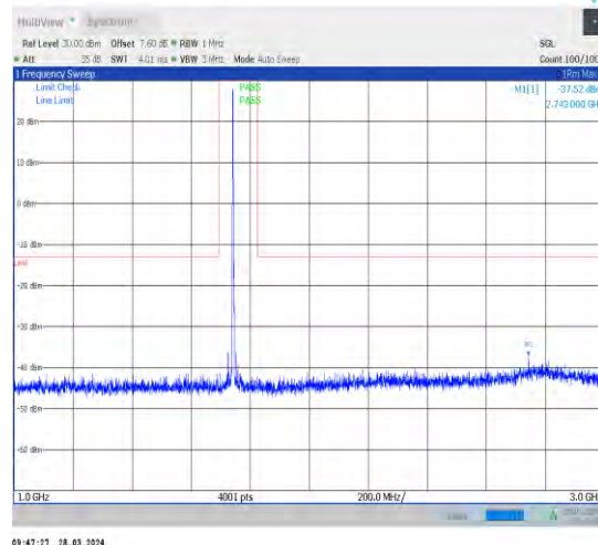
1-N66-15-40-H-1-DFT-PI2BPSK-Inner_1RB_Left-1@ 1-1000-3000-Ant1-2743.00--37.52--13-PASS
