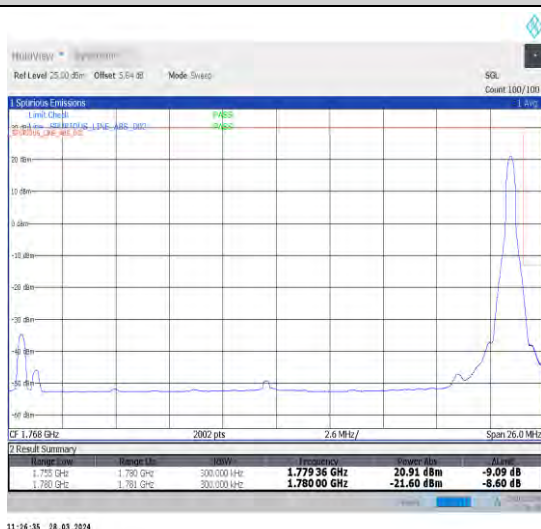
1-N66-15-25-H-5-CP-QPSK-Edge_1RB_Right-1@132-Ant1-1-seegraph-PASS-see graph
