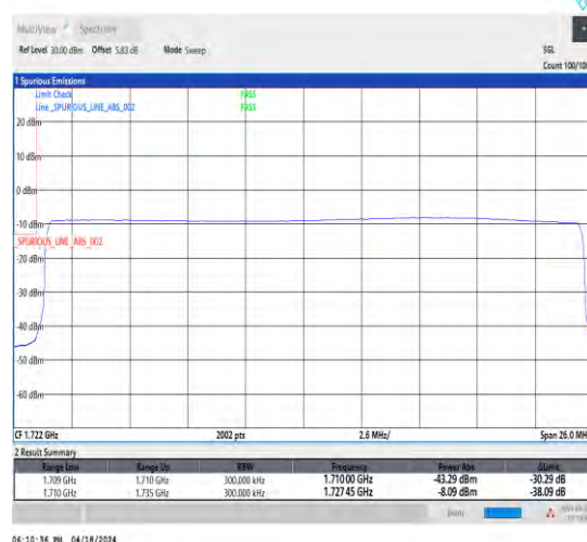
1-N66-15-25-L-6-CP-QPSK-Outer_Full-133@0-Ant1-1-seegraph-PASS-see graph
