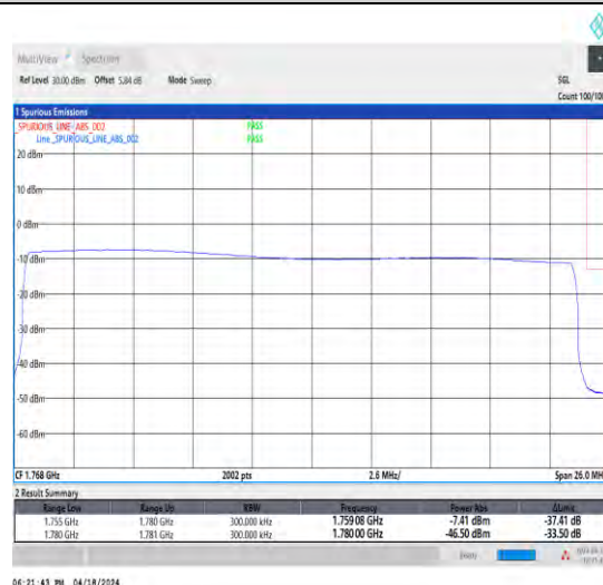
1-N66-15-25-H-6-CP-QPSK-Outer_Full-133@0-Ant1-1-seegraph-PASS-see graph
