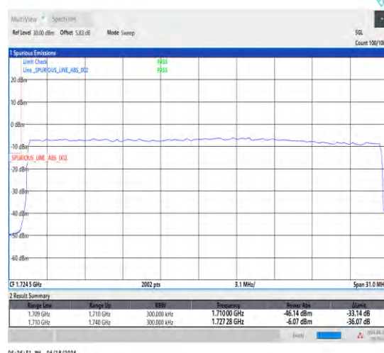
1-N66-15-30-L-3-DFT-PI2BPSK-Outer_Full-160@0-Ant1-1-seegraph-PASS-see graph
