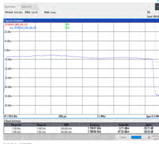
1-N66-15-30-H-3-DFT-PI2BPSK-Outer_Full-160@0-Ant1-1-seegraph-PASS-see graph
