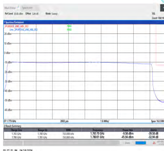
1-N66-15-15-H-6-CP-QPSK-Outer_Full-79@0-Ant1-1-seegraph-PASS-see graph
