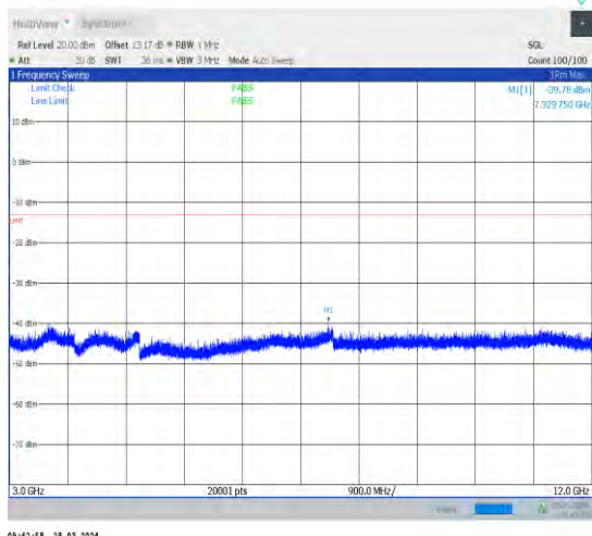
1-N66-15-40-L-1-DFT-PI2BPSK-Inner_1RB_Left-1 @ 1-3000-12000-Ant1-7929.75--39.78--13-PASS
