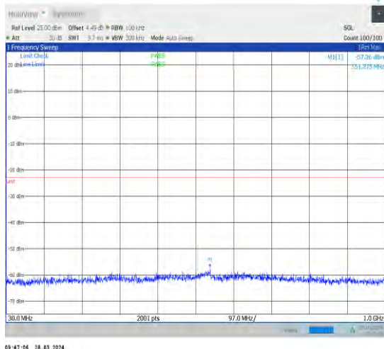
1-N66-15-40-H-1-DFT-PI2BPSK-Inner_1RB_Left-1 @1-30-1000-Ant1-551.38--57.36--23-PASS
