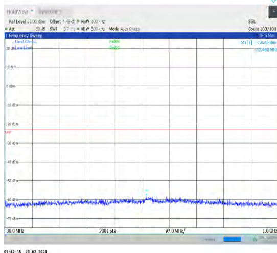
1-N66-15-40-L-1-DFT-PI2BPSK-Inner_1RB_Left-1 @1-30-1000-Ant1-532.46--58.45--23-PASS
