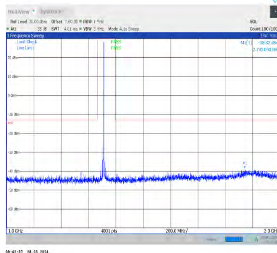
1-N66-15-40-L-1-DFT-PI2BPSK-Inner_1RB_Left-1@ 1-1000-3000-Ant1-2743.00--38.82--13-PASS
