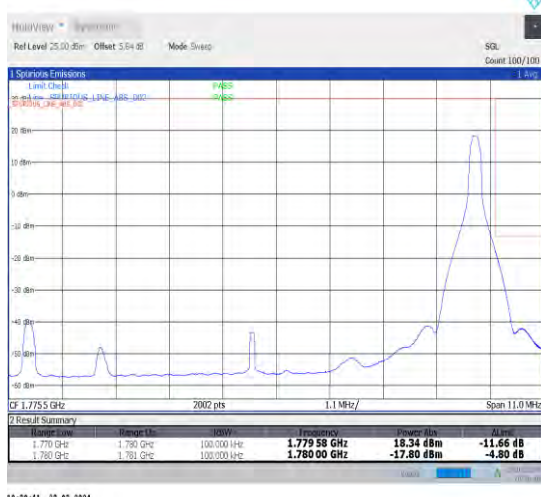
1-N66-15-10-H-5-CP-QPSK-Edge_1RB_Right-1@51-Ant1-1-seegraph-PASS-see graph
