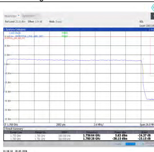
1-N66-15-25-H-3-DFT-PI2BPSK-Outer_Full-128@0-Ant1-1-seegraph-PASS-see graph
