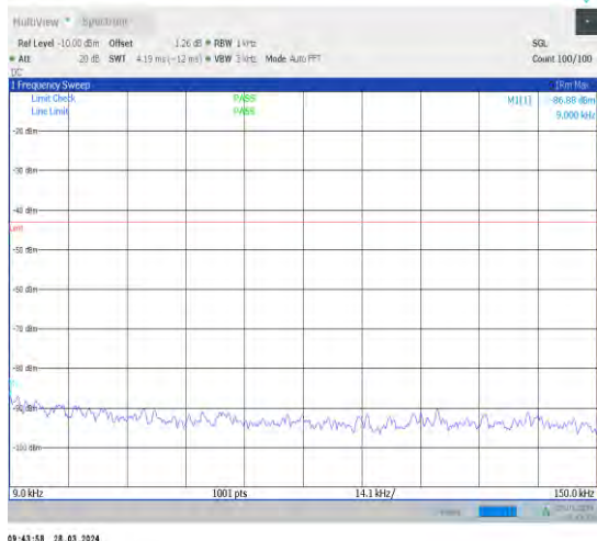
1-N66-15-40-M-1-DFT-PI2BPSK-Inner_1RB_Left-1 @ 1-0.009-0.15-Ant1-0.01--86.88--43-PASS
