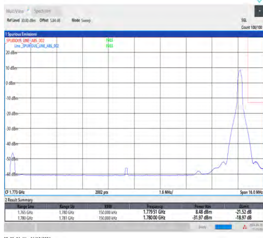
1-N66-15-15-H-2-DFT-PI2BPSK-Edge_1RB_Right-1@78-Ant1-1-seegraph-PASS-see graph
