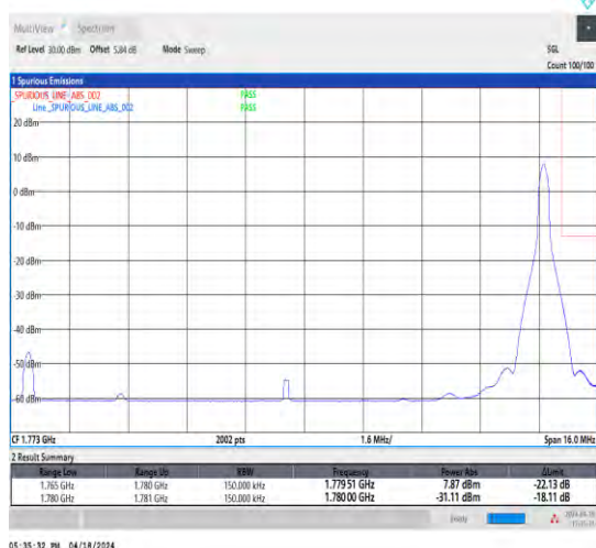
1-N66-15-15-H-5-CP-QPSK-Edge_1RB_Right-1@78-Ant1-1-seegraph-PASS-see graph
