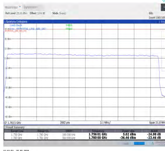
1-N66-15-30-H-3-DFT-PI2BPSK-Outer_Full-160@0-Ant1-1-seegraph-PASS-see graph
