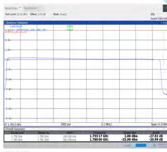
1-N66-15-30-H-6-CP-QPSK-Outer_Full-160@0-Ant1-1-seegraph-PASS-see graph
