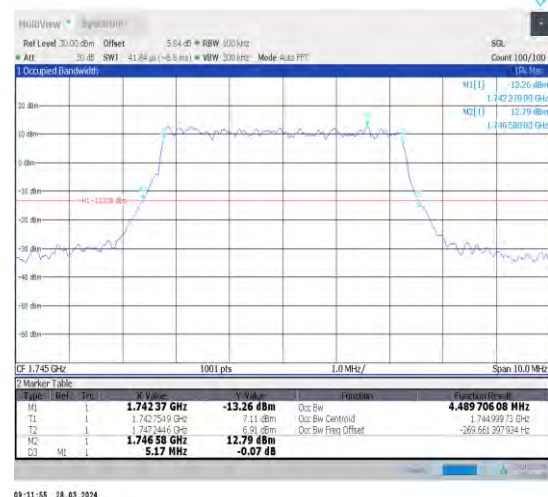
1-N66-15-5-M-8-CP-64QAM-Outer_Full-25@0-Ant1- 4.49-5.170-≤5-PASS
