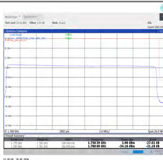
1-N66-15-25-H-6-CP-QPSK-Outer_Full-133@0-Ant1-1-seegraph-PASS-see graph
