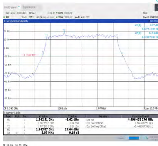
1-N66-15-5-M-2-DFT-PI2BPSK-Outer_Full-25@0-An t1-4.496-5.070-≤5-PASS
