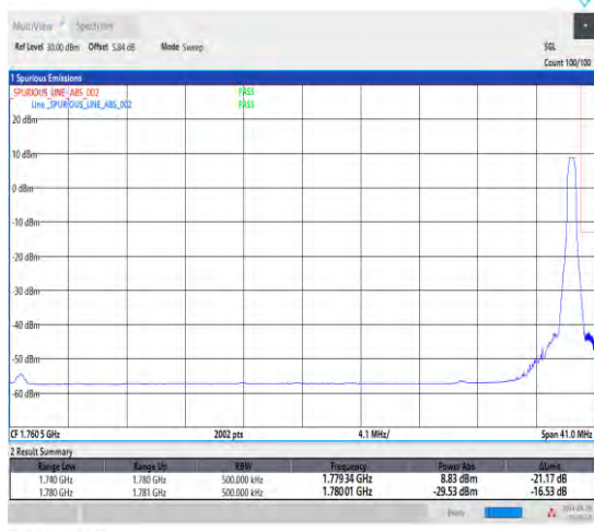
1-N66-15-40-H-5-CP-QPSK-Edge_1RB_Right-1@215-Ant1-1-seegraph-PASS-see graph
