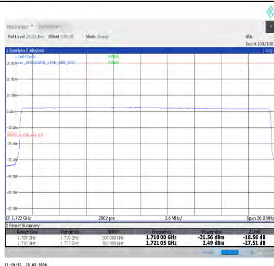
1-N66-15-25-L-6-CP-QPSK-Outer_Full-133@0-Ant1-1-seegraph-PASS-see graph
