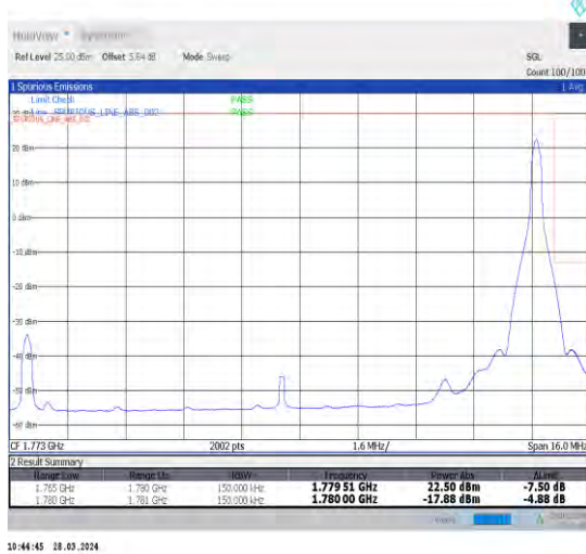
1-N66-15-15-H-2-DFT-PI2BPSK-Edge_1RB_Right-1@78-Ant1-1-seegraph-PASS-see graph
