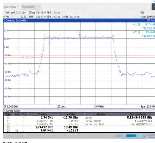
1-N66-15-10-M-1-DFT-QPSK-Outer_Full-50@0-Ant1 -8.925-9.640-≤10-PASS
