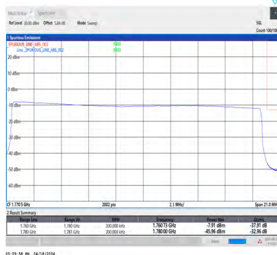
1-N66-15-20-H-6-CP-QPSK-Outer_Full-106@0-Ant1-1-seegraph-PASS-see graph
