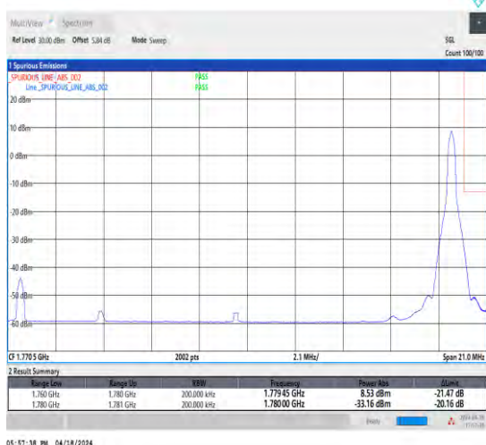
1-N66-15-20-H-5-CP-QPSK-Edge_1RB_Right-1@105-Ant1-1-seegraph-PASS-see graph
