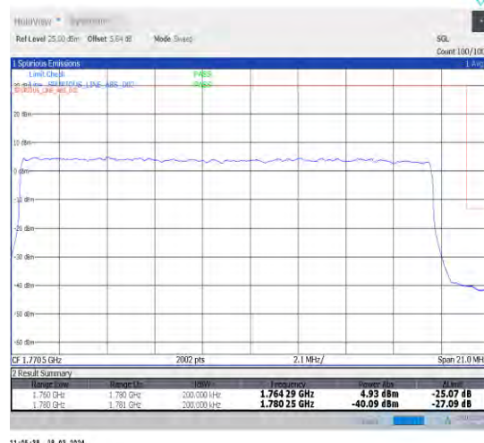
1-N66-15-20-H-3-DFT-PI2BPSK-Outer_Full-100@0-Ant1-1-seegraph-PASS-see graph
