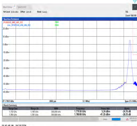
1-N66-15-30-H-5-CP-QPSK-Edge_1RB_Right-1@159-Ant1-1-seegraph-PASS-see graph
