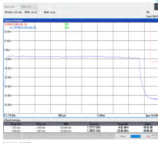
1-N66-15-15-H-3-DFT-PI2BPSK-Outer_Full-75@0-Ant1-1-seegraph-PASS-see graph
