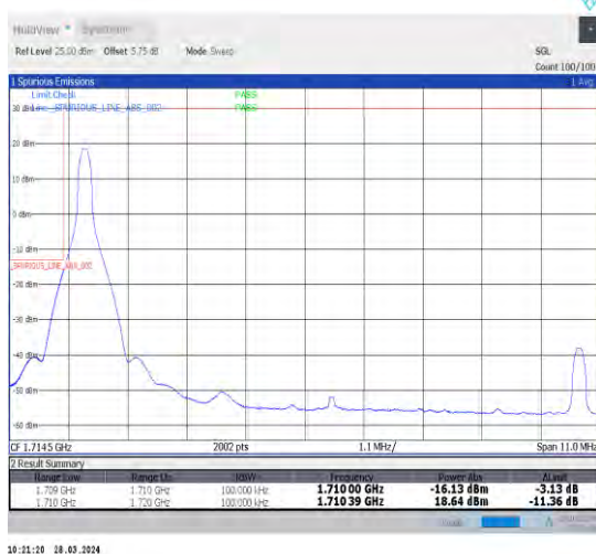
1-N66-15-10-L-4-CP-QPSK-Edge_1RB_Left-1@0-Ant1-1-seegraph-PASS-see graph
