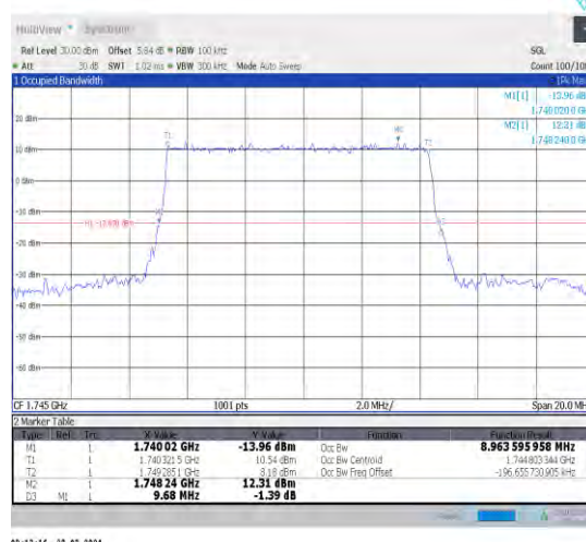
1-N66-15-10-M-3-DFT-16QAM-Outer_Full-50@0-Ant1 1-8.964-9.680-≤10-PASS
