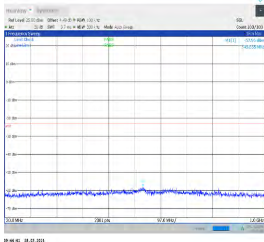
1-N66-15-40-M-1-DFT-PI2BPSK-Inner_1RB_Left-1 @ 1-30-1000-Ant1-545.56--57.96--23-PASS
