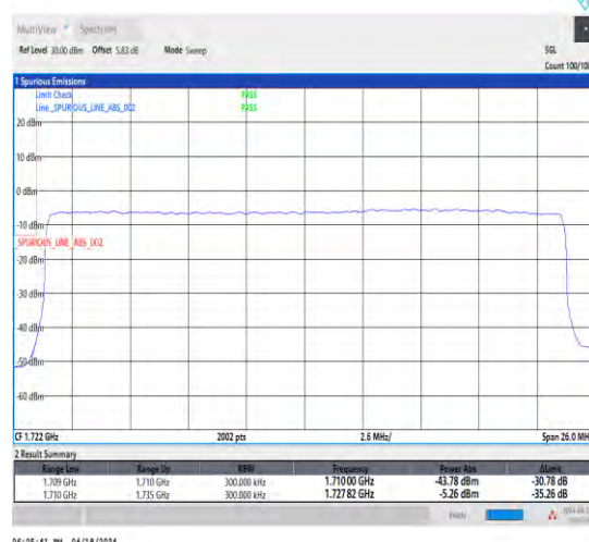
1-N66-15-25-L-3-DFT-PI2BPSK-Outer_Full-128@0-Ant1-1-seegraph-PASS-see graph
