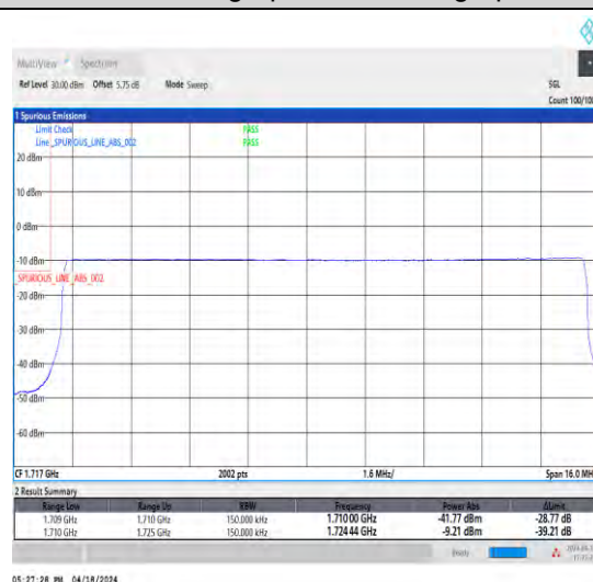
1-N66-15-15-L-6-CP-QPSK-Outer_Full-79@0-Ant1-1-seegraph-PASS-see graph
