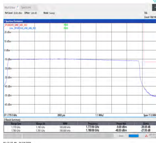
1-N66-15-10-H-6-CP-QPSK-Outer_Full-52@0-Ant1-1-seegraph-PASS-see graph
