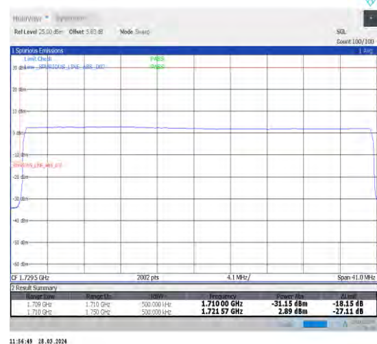
1-N66-15-40-L-6-CP-QPSK-Outer_Full-216@0-Ant1-1-seegraph-PASS-see graph
