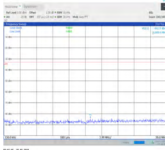
1-N66-15-40-H-1-DFT-PI2BPSK-Inner_1RB_Left-1@ 1-0.15-30-Ant1-16.00--84.17--33-PASS
