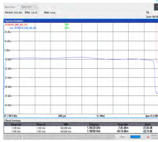
1-N66-15-40-H-6-CP-QPSK-Outer_Full-216@0-Ant1-1-seegraph-PASS-see graph
