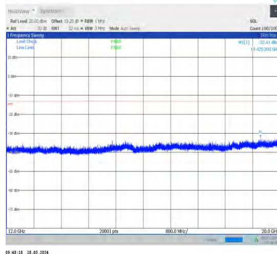
1-N66-15-40-H-1-DFT-PI2BPSK-Inner_1RB_Left-1@ 1-12000-20000-Ant1-19425.20--32.41--13-PASS
