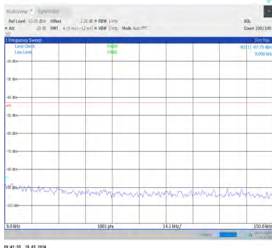
1-N66-15-40-L-1-DFT-PI2BPSK-Inner_1RB_Left-1 @1-0.009-0.15-Ant1-0.01--87.79--43-PASS
