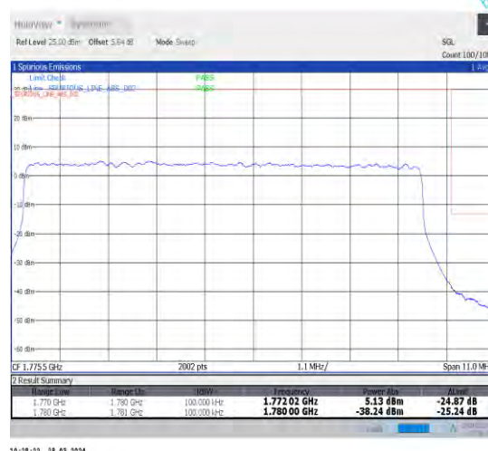
1-N66-15-10-H-3-DFT-PI2BPSK-Outer_Full-50@0-Ant1-1-seegraph-PASS-see graph
