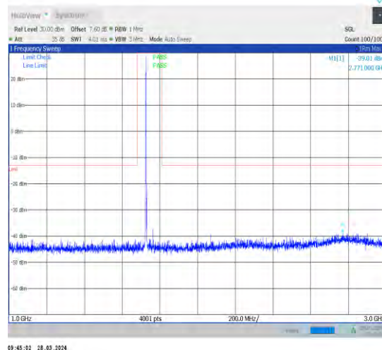
1-N66-15-40-M-1-DFT-PI2BPSK-Inner_1RB_Left-1@ 1-1000-3000-Ant1-2771.00--39.01--13-PASS
