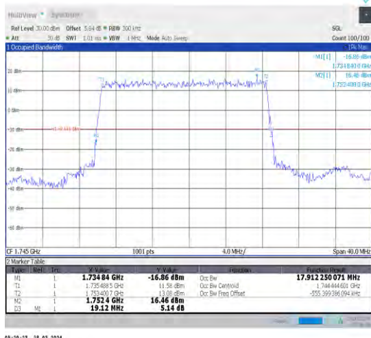
1-N66-15-20-M-2-DFT-PI2BPSK-Outer_Full-100@0-Ant1-17.912-19.120-≤20-PASS
