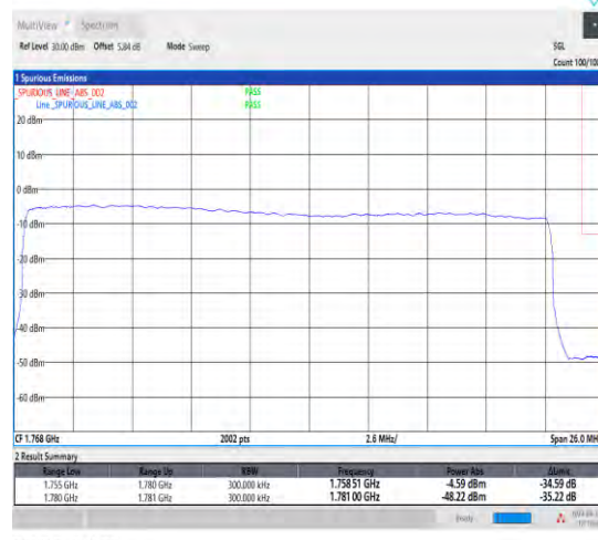
1-N66-15-25-H-3-DFT-PI2BPSK-Outer_Full-128@0-Ant1-1-seegraph-PASS-see graph
