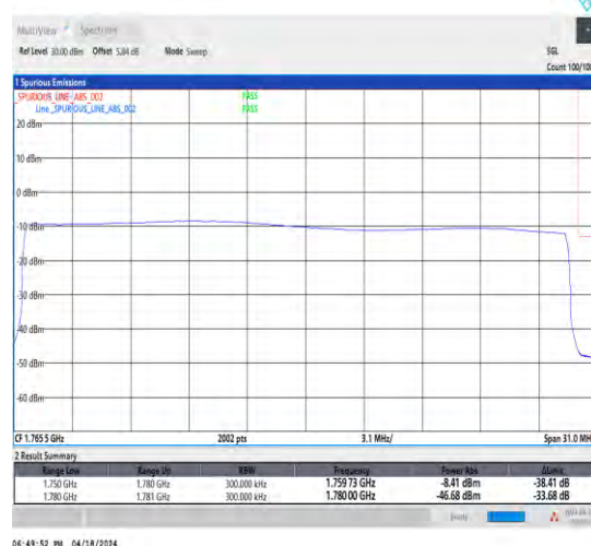
1-N66-15-30-H-6-CP-QPSK-Outer_Full-160@0-Ant1-1-seegraph-PASS-see graph
