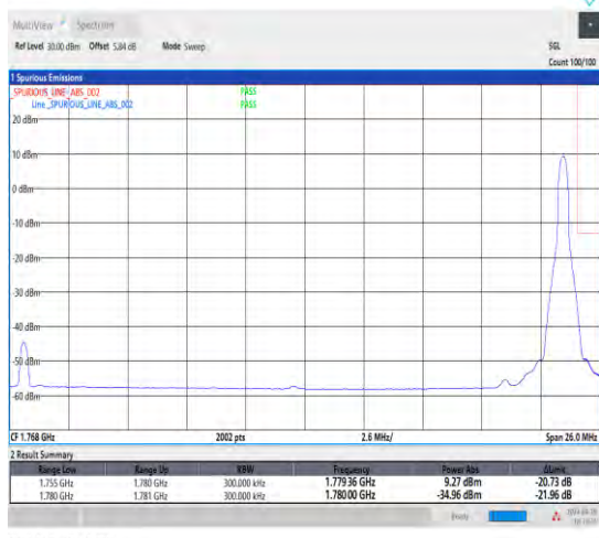
1-N66-15-25-H-2-DFT-PI2BPSK-Edge_1RB_Right-1@132-Ant1-1-seegraph-PASS-see graph
