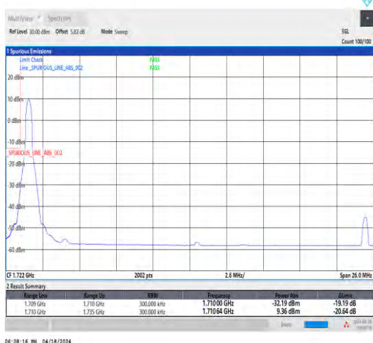
1-N66-15-25-L-4-CP-QPSK-Edge_1RB_Left-1@0-Ant1-1-seegraph-PASS-see graph
