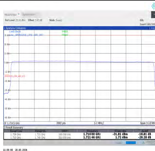
1-N66-15-30-L-6-CP-QPSK-Outer_Full-160@0-Ant1-1-seegraph-PASS-see graph
