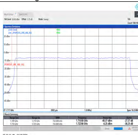
1-N66-15-15-L-3-DFT-PI2BPSK-Outer_Full-75@0-Ant1-1-seegraph-PASS-see graph
