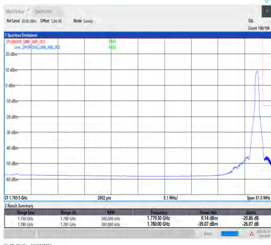
1-N66-15-30-H-2-DFT-PI2BPSK-Edge_1RB_Right-1@159-Ant1-1-seegraph-PASS-see graph
