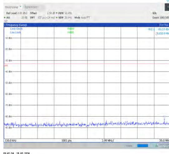
1-N66-15-40-L-1-DFT-PI2BPSK-Inner_1RB_Left-1@ 1-0.15-30-Ant1-28.84--83.53--33-PASS
