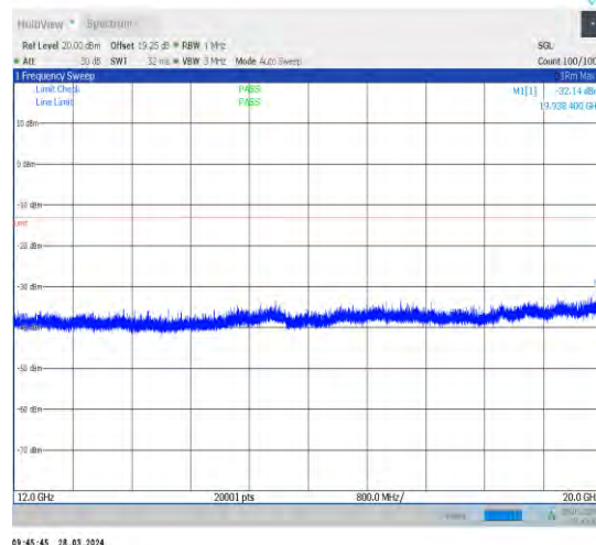
1-N66-15-40-M-1-DFT-PI2BPSK-Inner_1RB_Left-1@ 1-12000-20000-Ant1-19938.40--32.14--13-PASS
