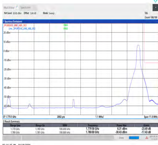
1-N66-15-10-H-5-CP-QPSK-Edge_1RB_Right-1@51-Ant1-1-seegraph-PASS-see graph
