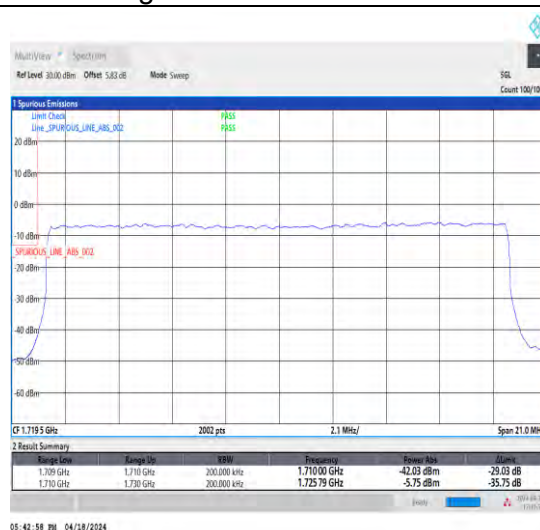
1-N66-15-20-L-3-DFT-PI2BPSK-Outer_Full-100@0-Ant1-1-seegraph-PASS-see graph
