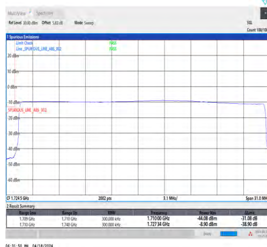
1-N66-15-30-L-6-CP-QPSK-Outer_Full-160@0-Ant1-1-seegraph-PASS-see graph
