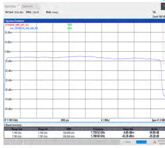
1-N66-15-40-H-3-DFT-PI2BPSK-Outer_Full-216@0-Ant1-1-seegraph-PASS-see graph
