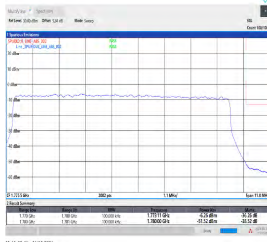
1-N66-15-10-H-3-DFT-PI2BPSK-Outer_Full-50@0-Ant1-1-seegraph-PASS-see graph
