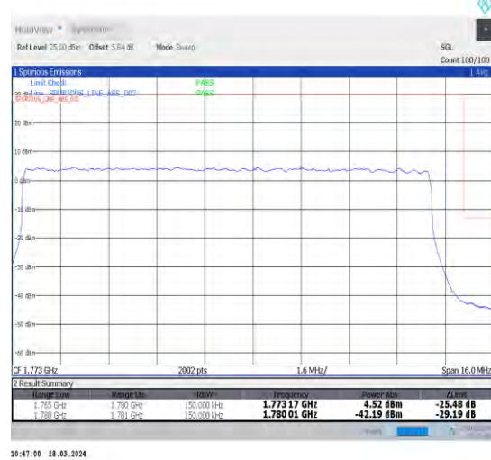
1-N66-15-15-H-3-DFT-PI2BPSK-Outer_Full-75@0-Ant1-1-seegraph-PASS-see graph
