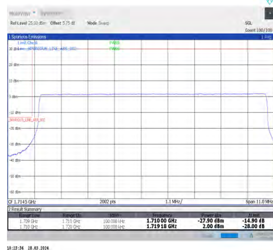
1-N66-15-10-L-6-CP-QPSK-Outer_Full-52@0-Ant1-1-seegraph-PASS-see graph
