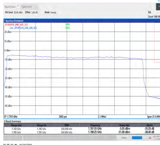
1-N66-15-20-H-3-DFT-PI2BPSK-Outer_Full-100@0-Ant1-1-seegraph-PASS-see graph
