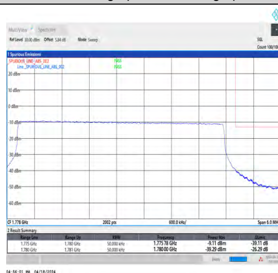
1-N66-15-5-H-6-CP-QPSK-Outer_Full-25@0-Ant1-1-seegraph-PASS-see graph
