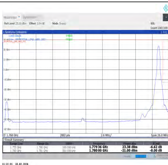
1-N66-15-25-H-2-DFT-PI2BPSK-Edge_1RB_Right-1@132-Ant1-1-seegraph-PASS-see graph
