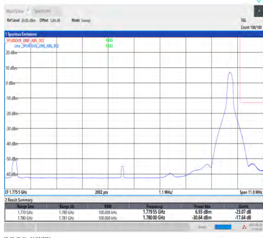
1-N66-15-10-H-2-DFT-PI2BPSK-Edge_1RB_Right-1@51-Ant1-1-seegraph-PASS-see graph
