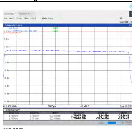
1-N66-15-40-H-3-DFT-PI2BPSK-Outer_Full-216@0-Ant1-1-seegraph-PASS-see graph
