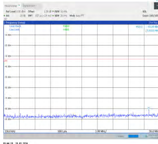
1-N66-15-40-M-1-DFT-PI2BPSK-Inner_1RB_Left-1@ 1-0.15-30-Ant1-27.91--82.50--33-PASS
