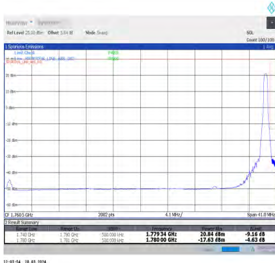
1-N66-15-40-H-5-CP-QPSK-Edge_1RB_Right-1@215-Ant1-1-seegraph-PASS-see graph
