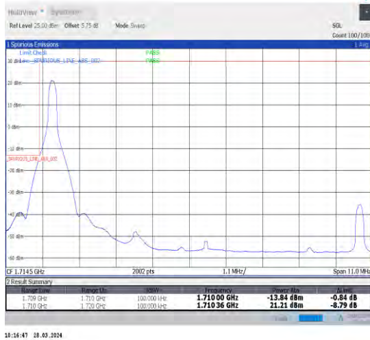
1-N66-15-10-L-1-DFT-PI2BPSK-Edge_1RB_Left-1@0-Ant1-1-seegraph-PASS-see graph
