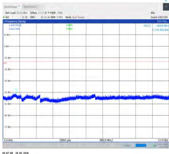
1-N66-15-40-H-1-DFT-PI2BPSK-Inner_1RB_Left-1 @1-3000-12000-Ant1-3716.40--40.68--13-PASS
