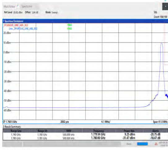
1-N66-15-40-H-2-DFT-PI2BPSK-Edge_1RB_Right-1@215-Ant1-1-seegraph-PASS-see graph
