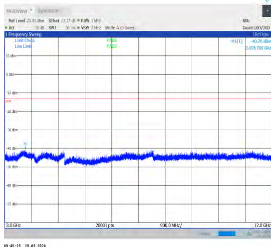
1-N66-15-40-M-1-DFT-PI2BPSK-Inner_1RB_Left-1 @ 1-3000-12000-Ant1-3695.70--40.76--13-PASS
