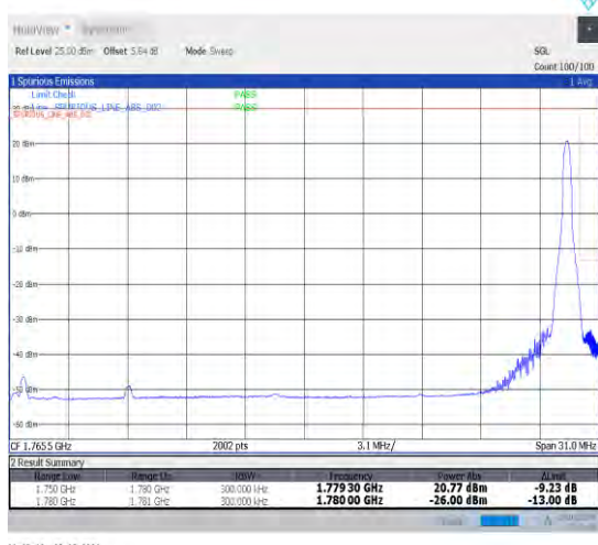
1-N66-15-30-H-5-CP-QPSK-Edge_1RB_Right-1@159-Ant1-1-seegraph-PASS-see graph
