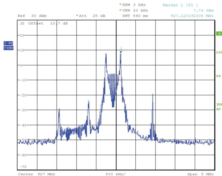
Figure 23 – Mid Channel Power Spectral Density (FSK)
