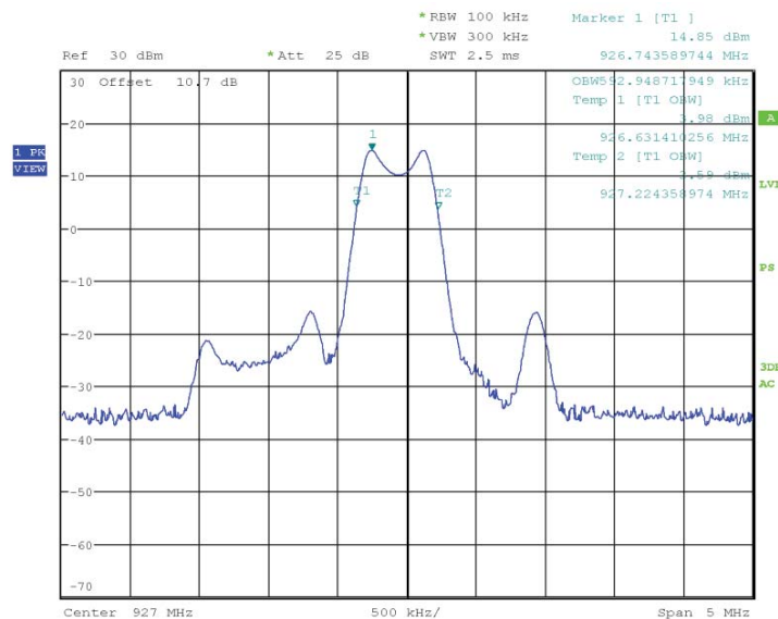
Figure 17 – Mid Channel 99% Occupied Bandwidth (FSK)
