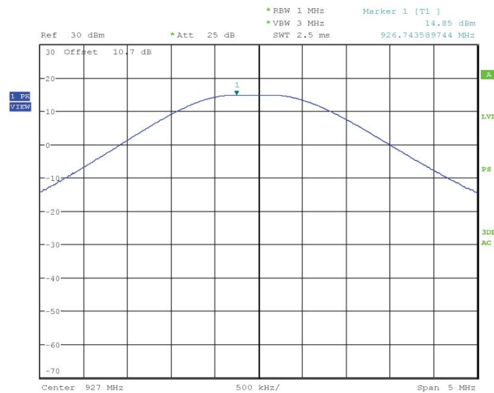
Figure 5 – Mid Channel Output Power (FSK)
