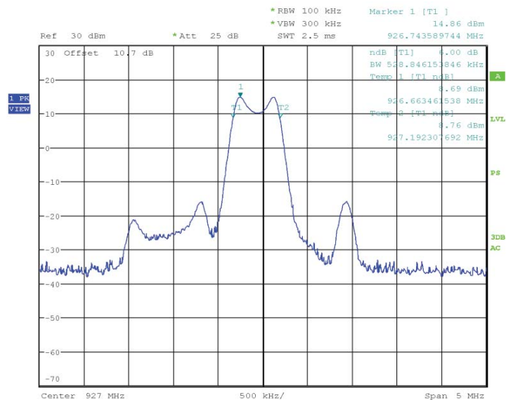
Figure 11 – Mid Channel 6 dB Occupied Bandwidth (FSK)
