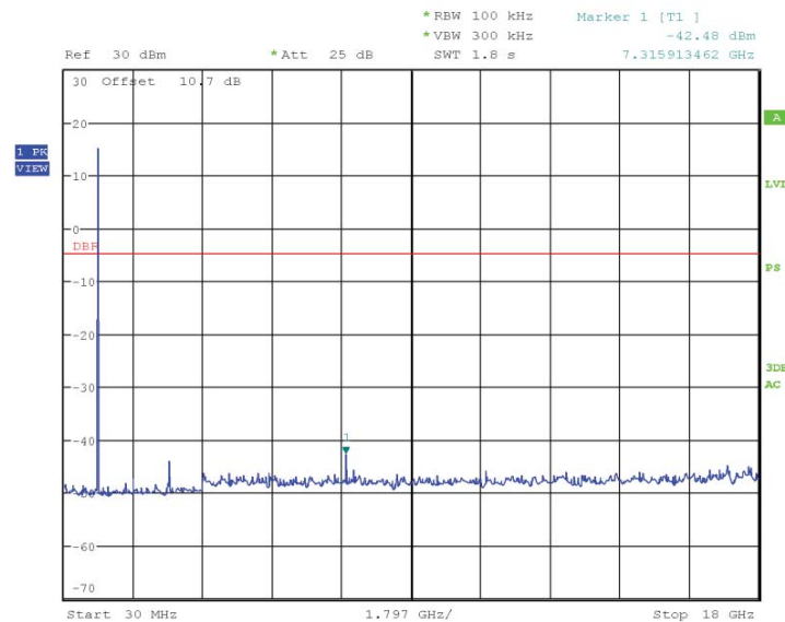
Figure 25 – Low Channel Conducted Spurious Emissions (LoRa)
