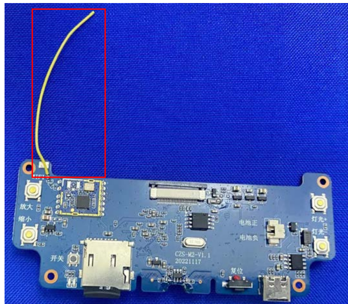
Antenna picture
