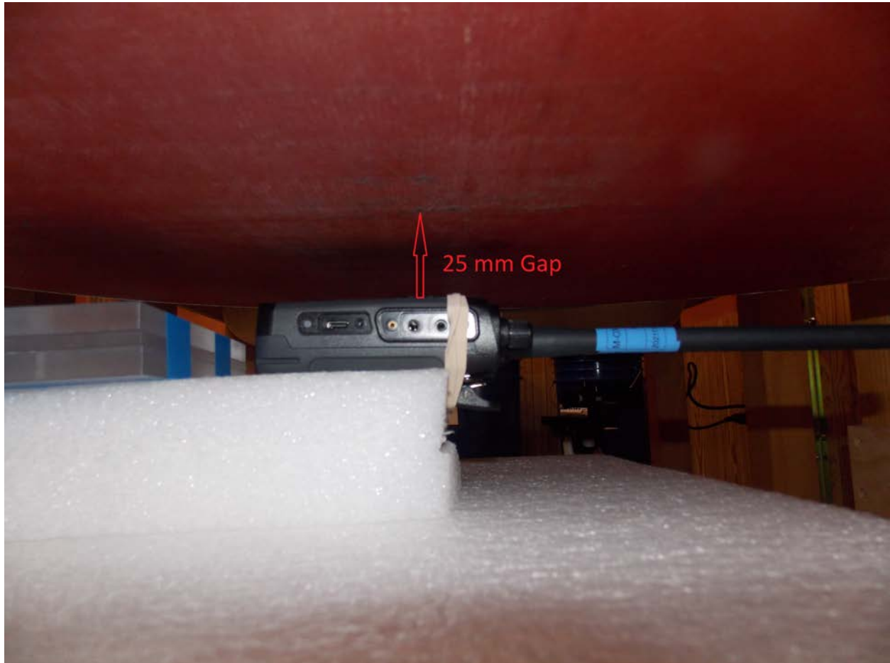
Face Test Position with 25 mm Gap
