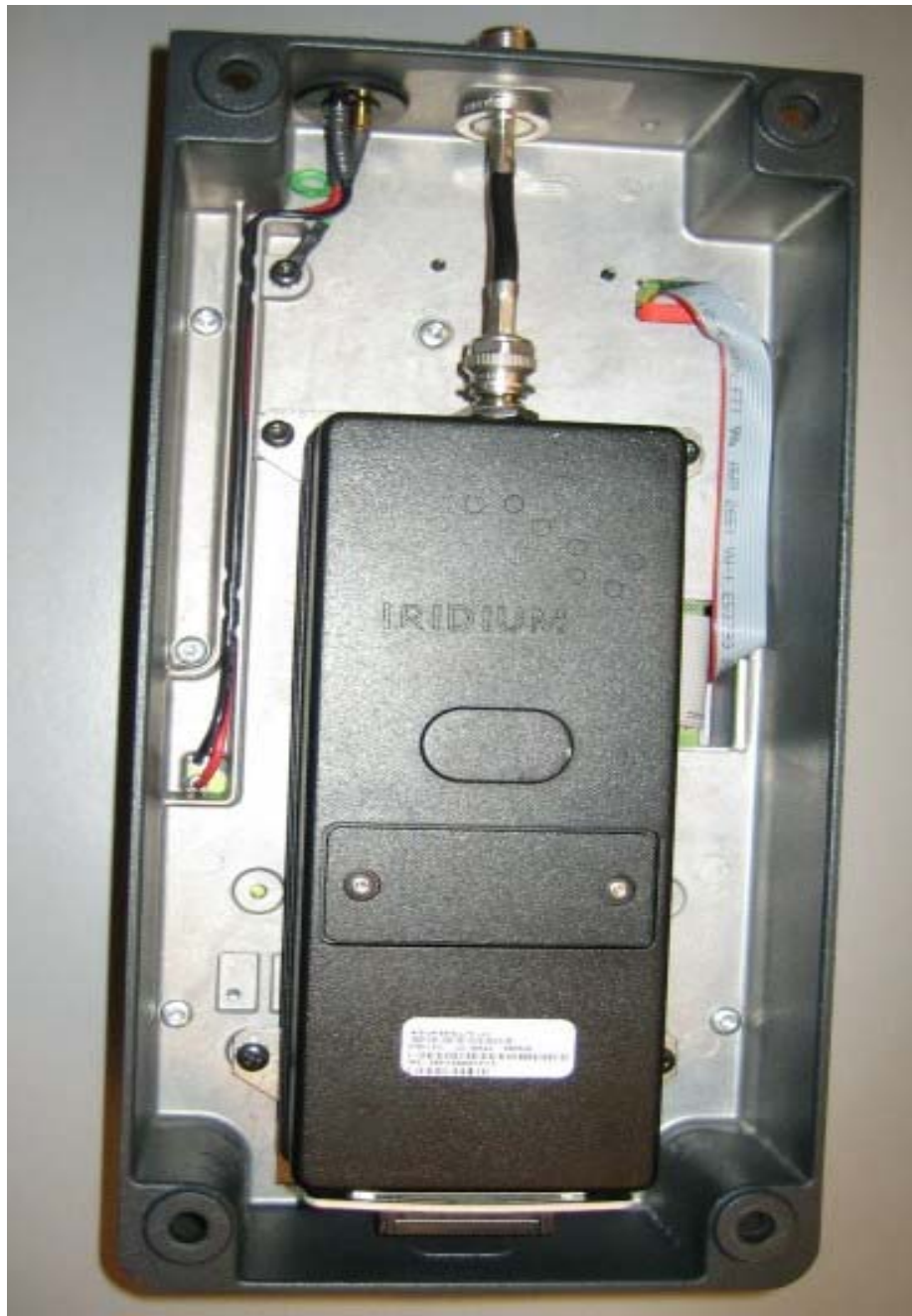
Internal of transceiver unit
