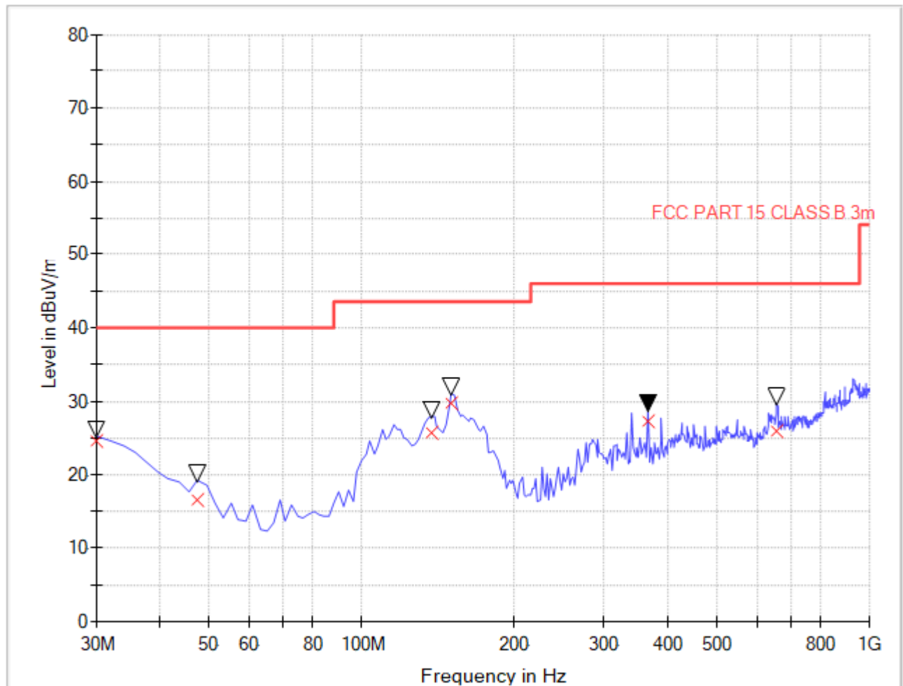
(Plot C: Test Antenna Horizontal 30M - 1G)
