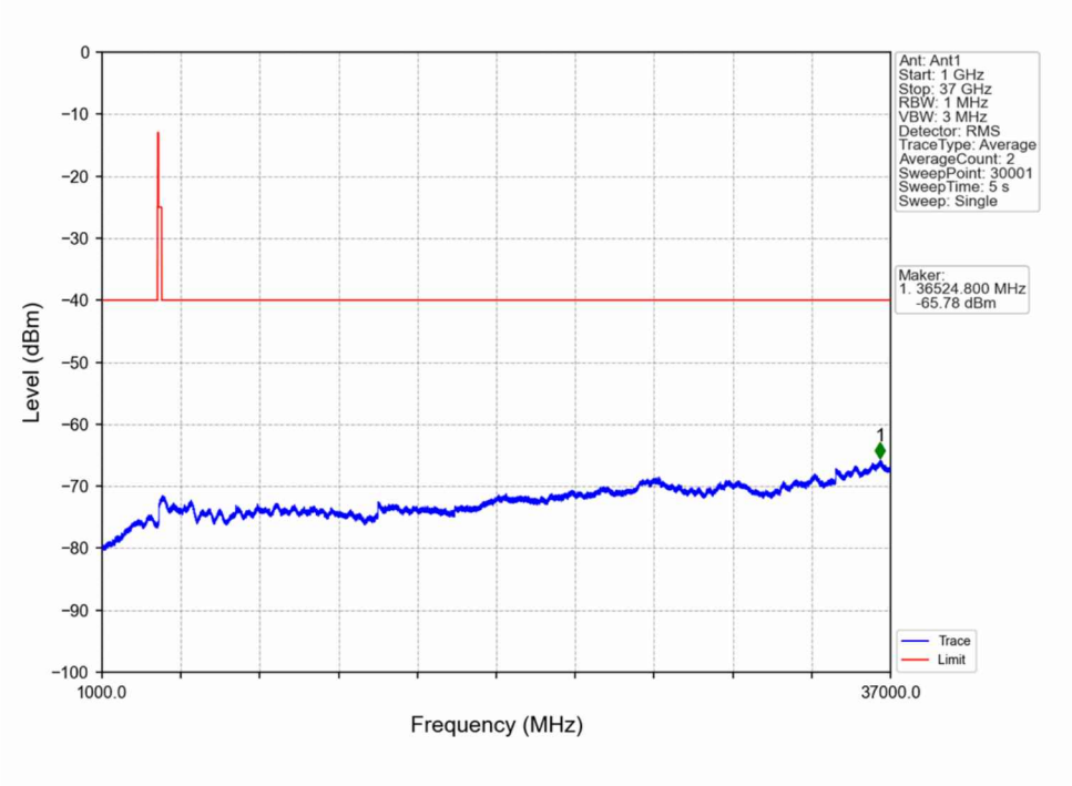
n48_30kHz_SISO_NTNV_10MHz_DFT-s-OFDM QPSK_3555MHz_Outer_Full
