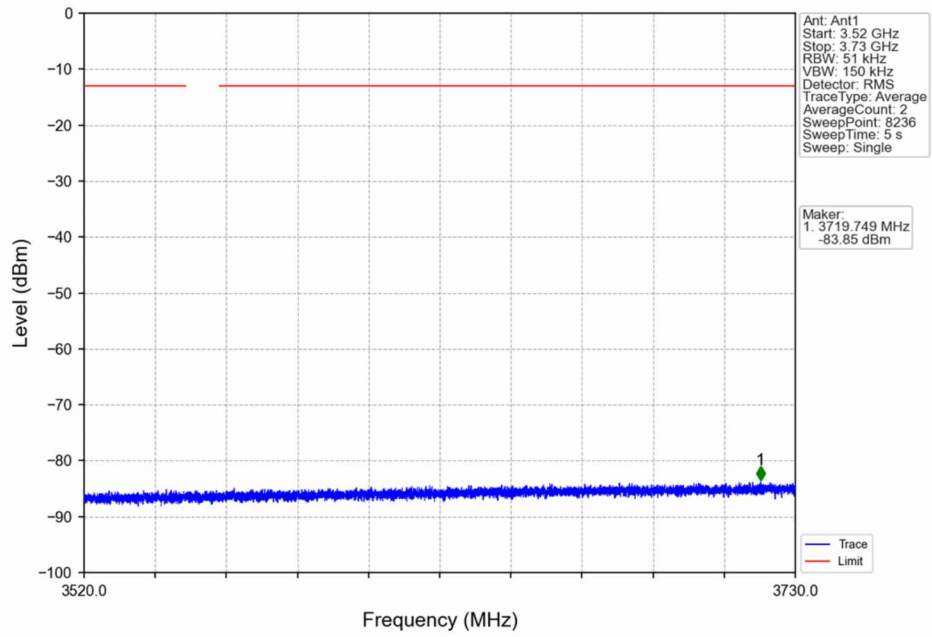
n48_30kHz_SISO_NTNV_10MHz_DFT-s-OFDM QPSK_3555MHz_Outer_Full
