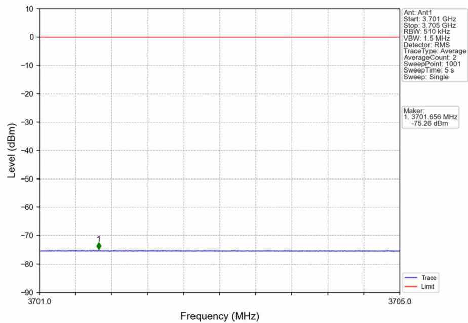
n48_30kHz_SISO_NTNV_10MHz_DFT-s-OFDM QPSK_3694.98MHz_Inner_1RB_Right
