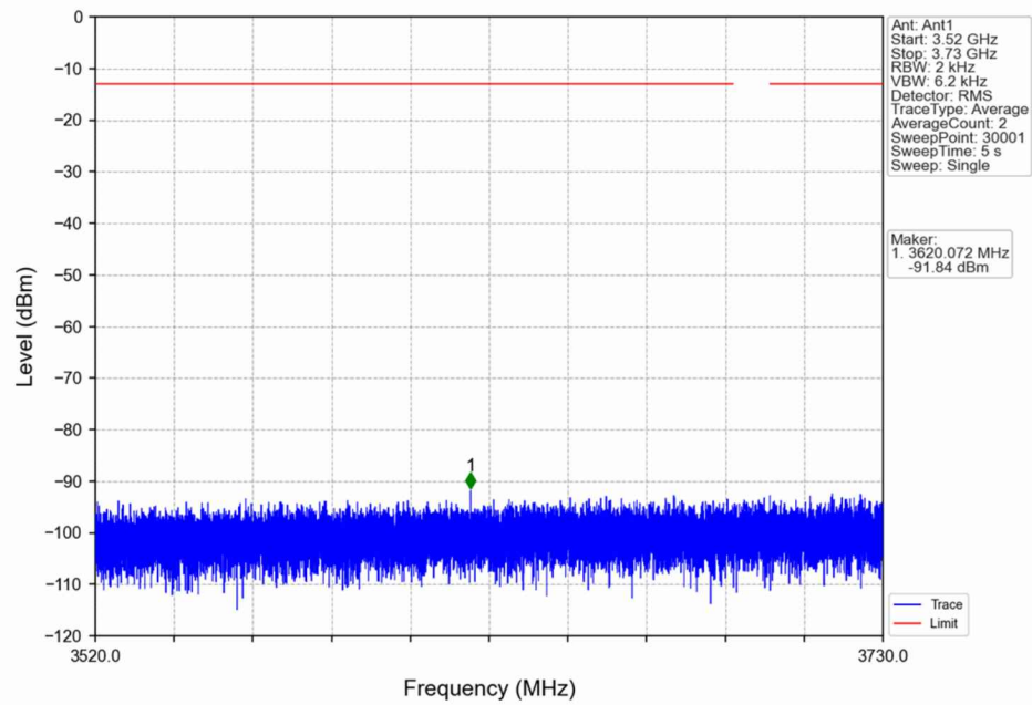
n48_30kHz_SISO_NTNV_10MHz_DFT-s-OFDM QPSK_3694.98MHz_Inner_1RB_Right
