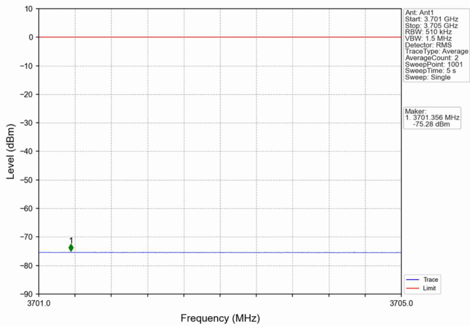
n48_30kHz_SISO_NTNV_10MHz_DFT-s-OFDM QPSK_3694.98MHz_Outer_Full
