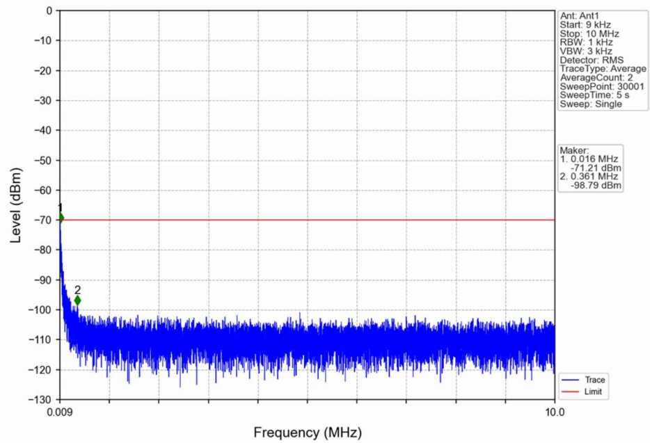
n48_30kHz_SISO_NTNV_10MHz_DFT-s-OFDM QPSK_3694.98MHz_Inner_1RB_Right
