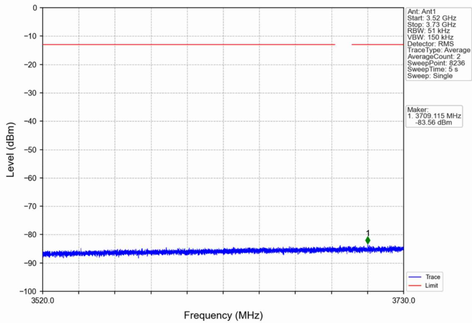
n48_30kHz_SISO_NTNV_10MHz_DFT-s-OFDM QPSK_3694.98MHz_Outer_Full
