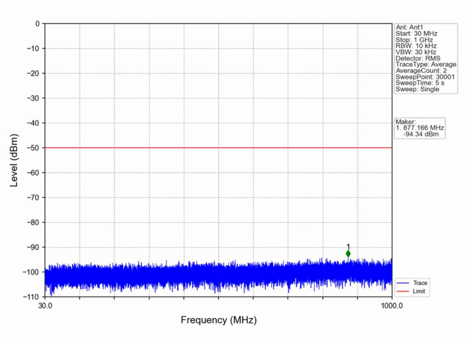
n48_30kHz_SISO_NTNV_10MHz_DFT-s-OFDM QPSK_3694.98MHz_Outer_Full
