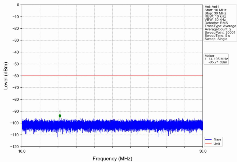
n48_30kHz_SISO_NTNV_10MHz_DFT-s-OFDM QPSK_3624.99MHz_Edge_1RB_Left
