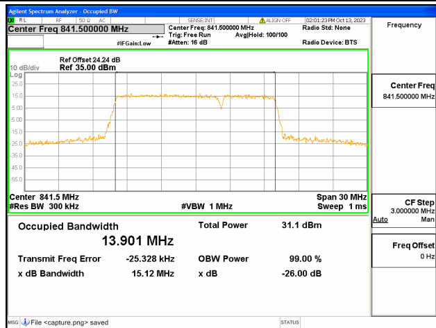
5B / 10+5MHz / QPSK/ High CH
