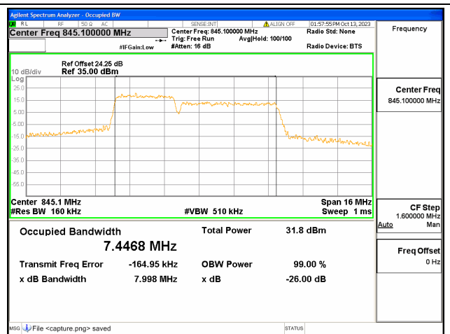
5B / 3+5MHz / 256QAM/ High CH
