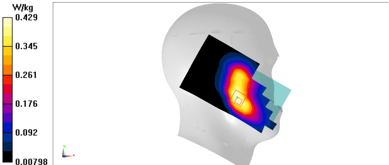
Fig.3 1900 MHz
