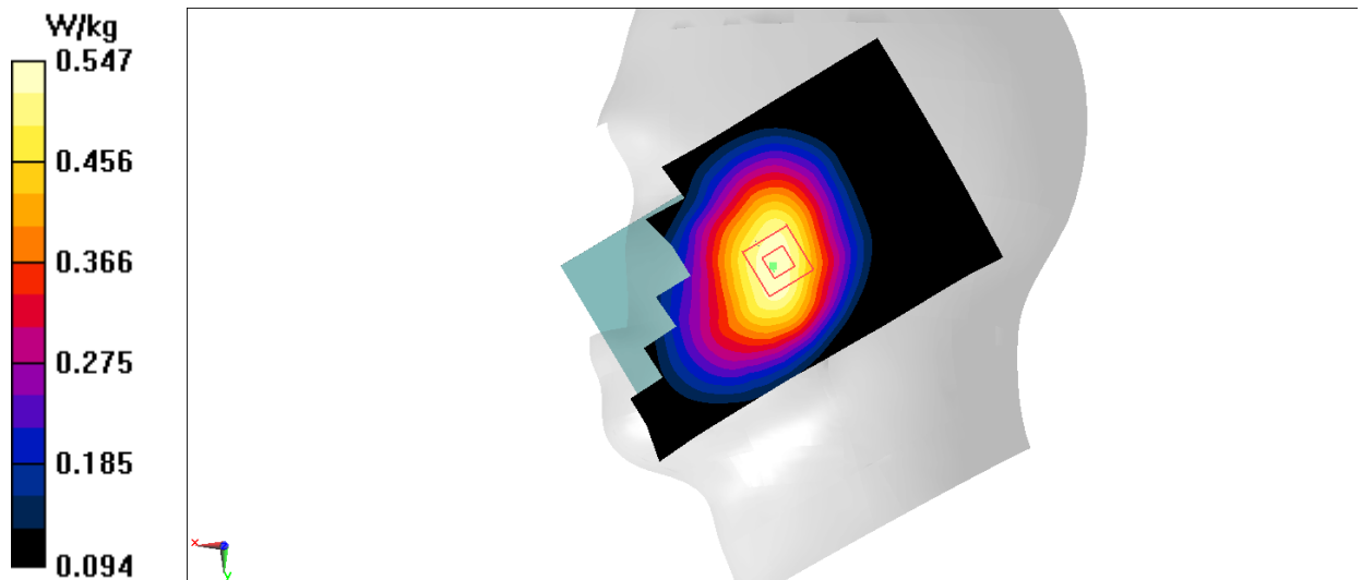
Fig.1 850MHz
