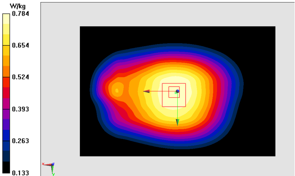
Fig.2 850 MHz
