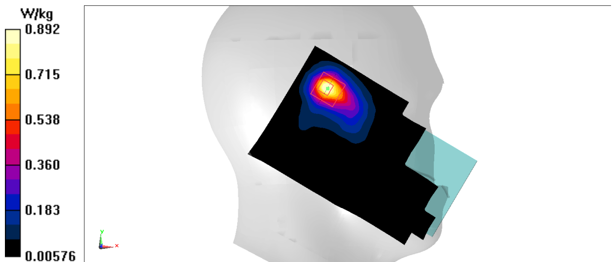
Fig.13 2450 MHz
