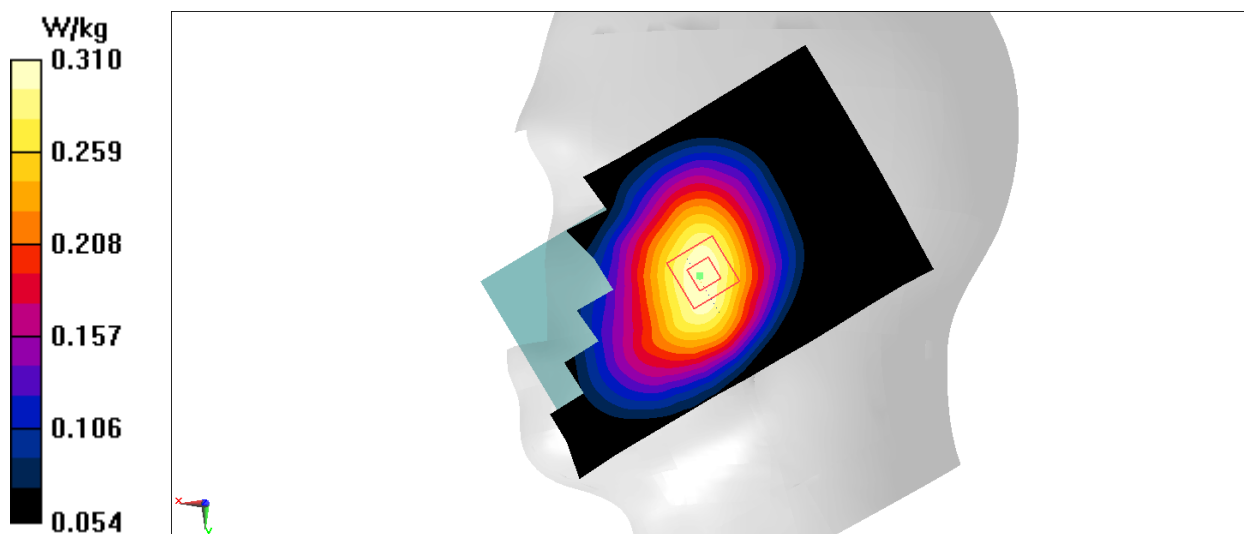
Fig.7 LTE Band5
