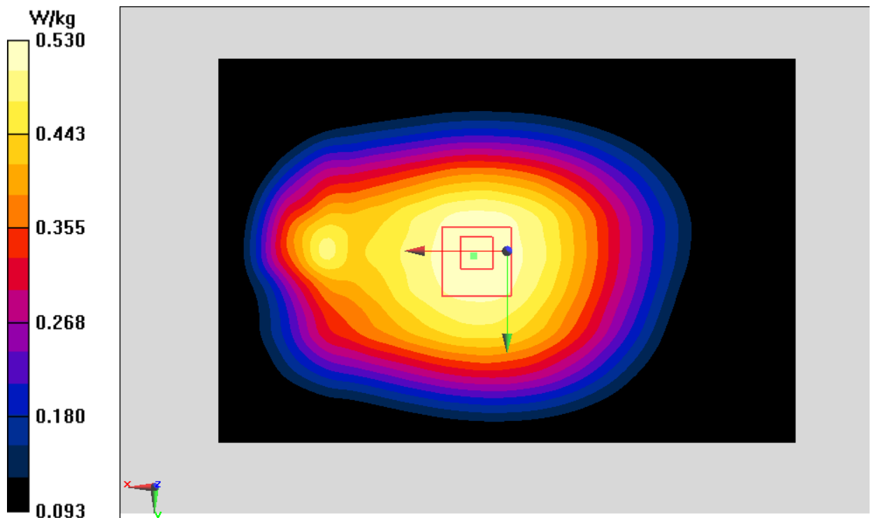
Fig.8 LTE Band5
