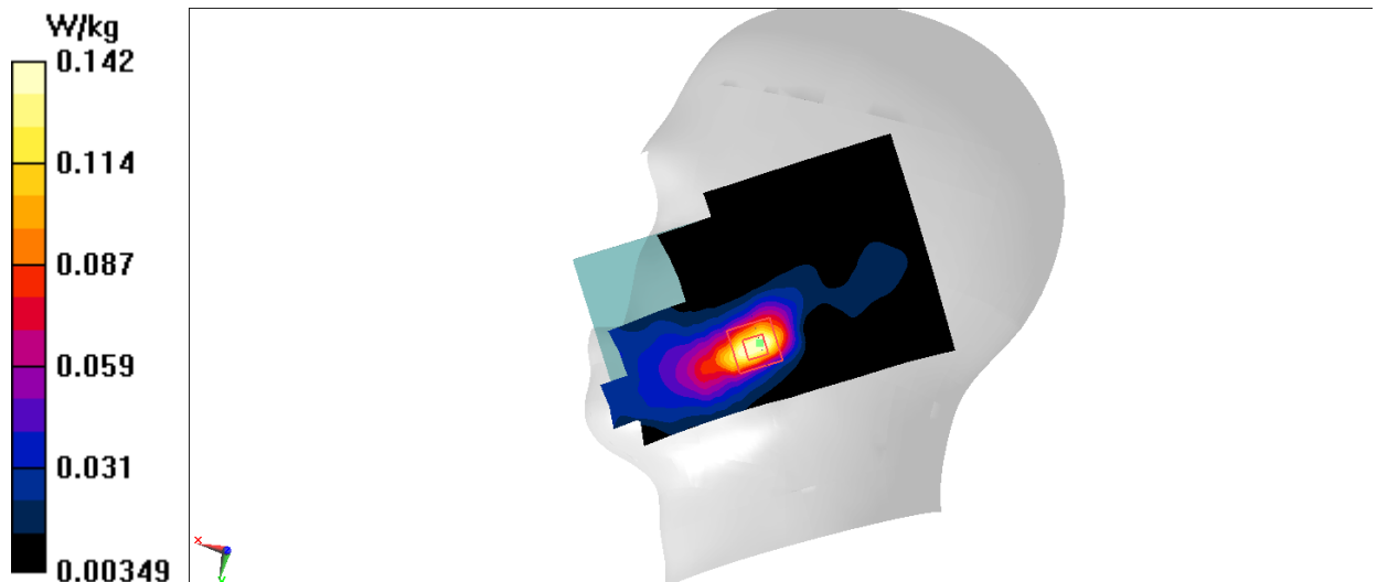
Fig.11 LTE Band 38
