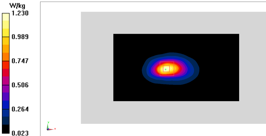
Fig.4 1900 MHz
