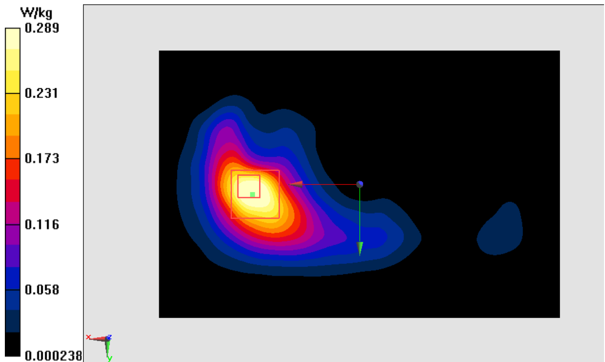
Fig.12 LTE Band 38
