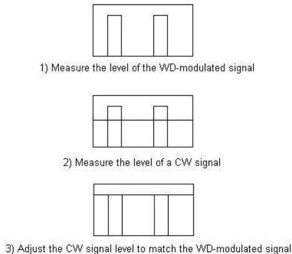
Figure 3: Setting the RF levels for determining the PMF (0 Hz span plots). The CW signal amplitude is adjusted to match the peak of the WD-modulated signal.
