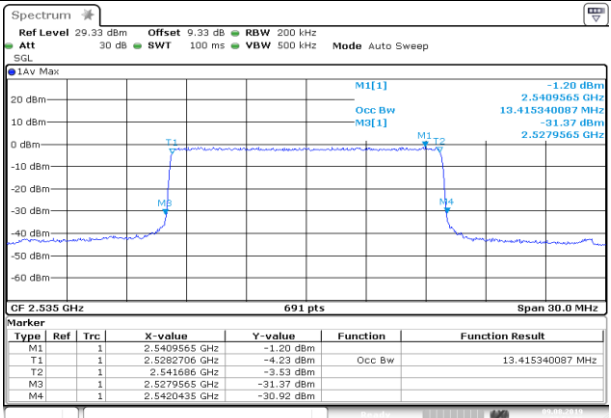
MCH_16QAM_75RB#0
