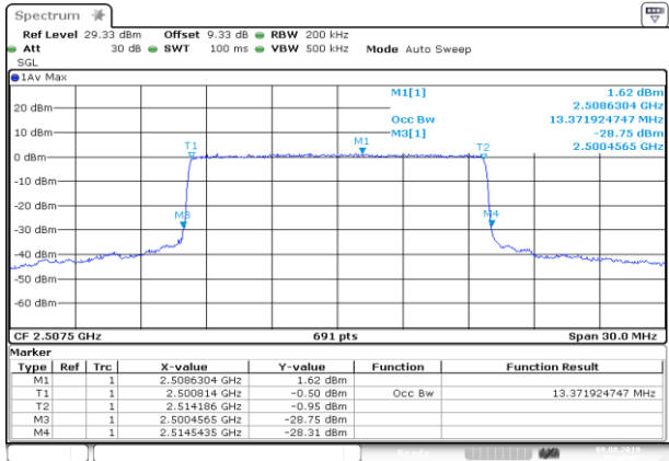
LCH_QPSK_75RB#0
