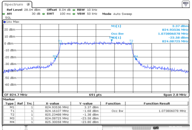
LCH_16QAM_6RB#0
