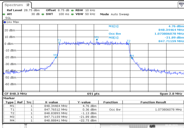
HCH_QPSK_6RB#0
