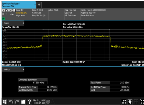
B5_N78(70M)_CP- OFDM_QPSK_Outer_Full_Mid_CH
