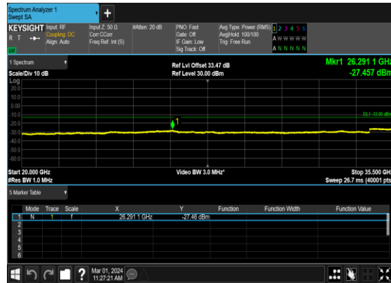
B5_N78(70M)_DFT-s- OFDM_QPSK_Edge_1RB_Left_Mid_CH
