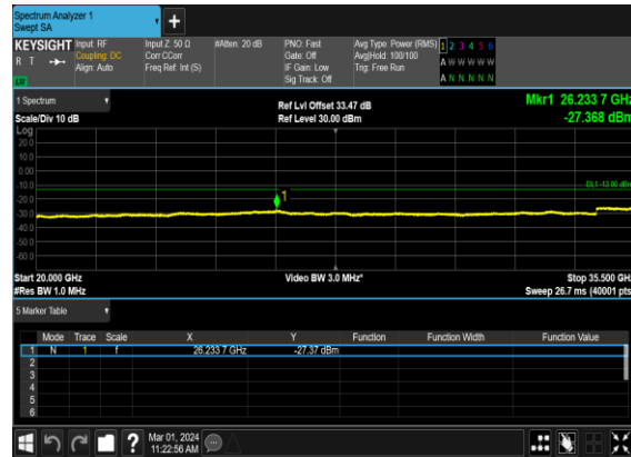
B5_N78(70M)_DFT-s-OFDM_BPSK_Edge_1RB_Left_Low_CH
