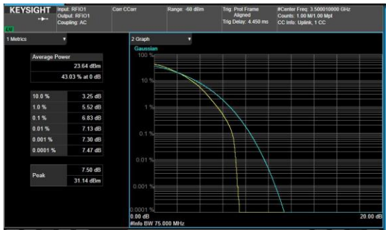
B5_N78(70M)_DFT-s-OFDM_QPSK_1RB_Left Mid CH
