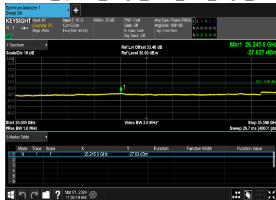
B5_N78(70M)_DFT-s- OFDM_QPSK_Edge_1RB_Left_High_CH
