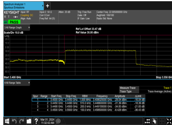
B5_N78(70M)_DFT-s- OFDM_QPSK_Outer_Full_Low_CH
