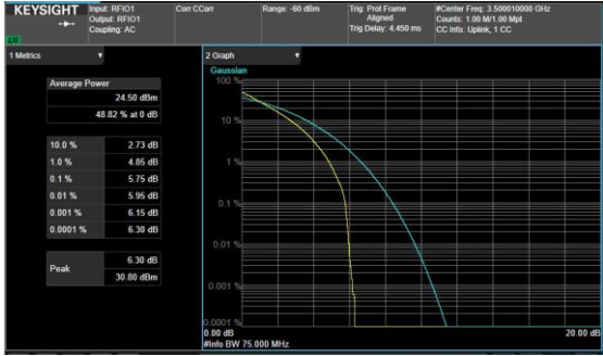
B5_N78(70M)_DFT-s-OFDM_PI_2- BPSK_1RB_Left_Mid_CH
