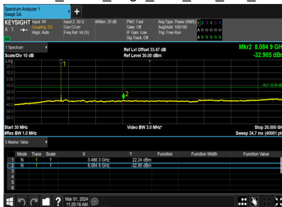
B5_N78(70M)_DFT-s-OFDM_BPSK_Edge_1RB_Left_Mid_CH
