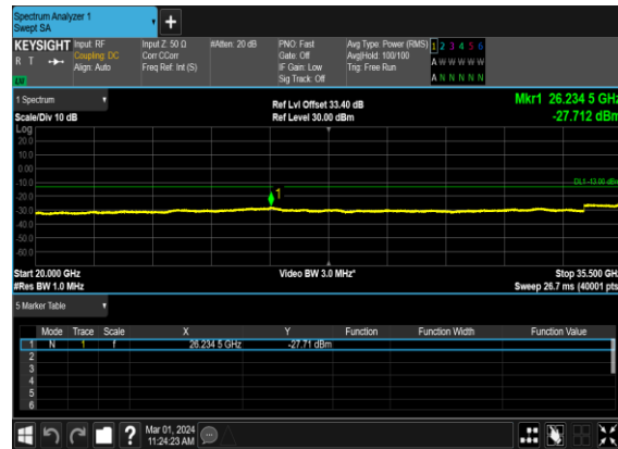
B5_N78(70M)_DFT-s-OFDM_QPSK_Edge_1RB_Left_Low_CH
