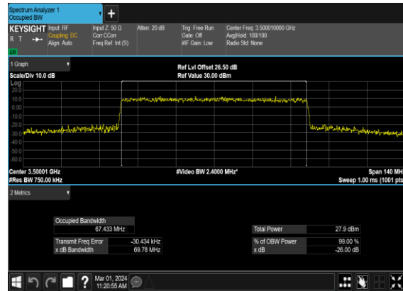
B5_N78(70M)_CP-OFDM_16 QAM_Outer_Full_Mid_CH
