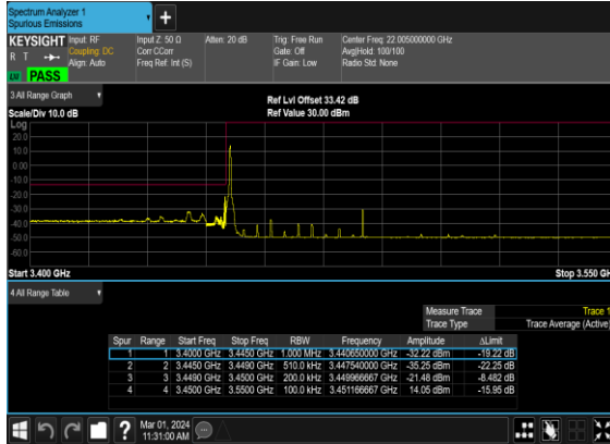
B5_N78(70M)_DFT-s- OFDM_BPSK_Edge_1RB_Left_Low_CH
