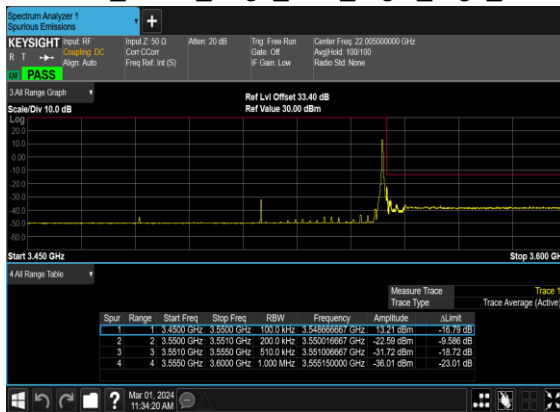
B5_N78(70M)_DFT-s- OFDM_BPSK_Edge_1RB_Right_High_CH
