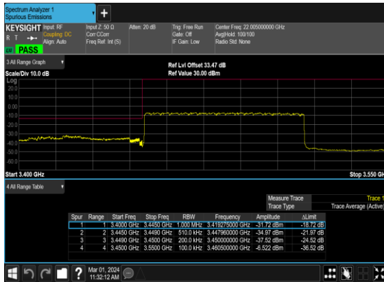
B5_N78(70M)_DFT-s- OFDM_BPSK_Outer_Full_Low_CH
