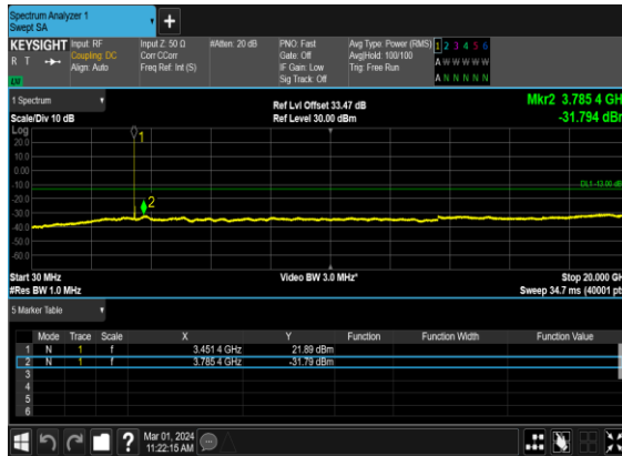
B5_N78(70M)_DFT-s-OFDM_BPSK_Edge_1RB_Left_Low_CH
