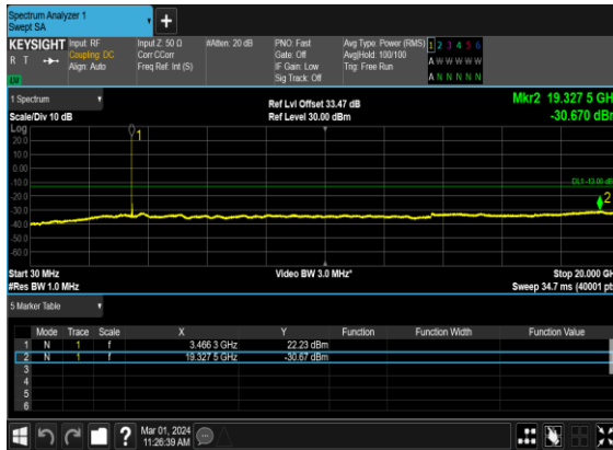
B5_N78(70M)_DFT-s- OFDM_QPSK_Edge_1RB_Left_Mid_CH
