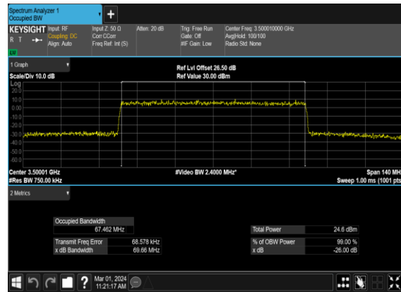
B5_N78(70M)_CP-OFDM_256 QAM_Outer_Full_Mid_CH
