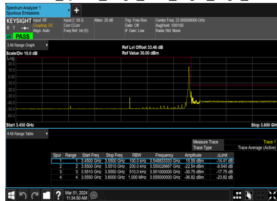
B5_N78(70M)_DFT-s- OFDM_QPSK_Edge_1RB_Right_High_CH
