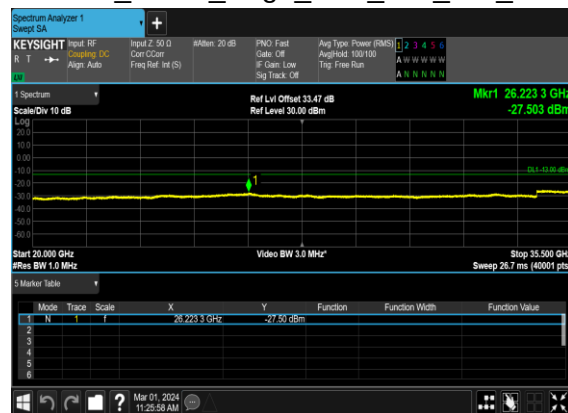
B5_N78(70M)_DFT-s-OFDM_BPSK_Edge_1RB_Left_Mid_CH
