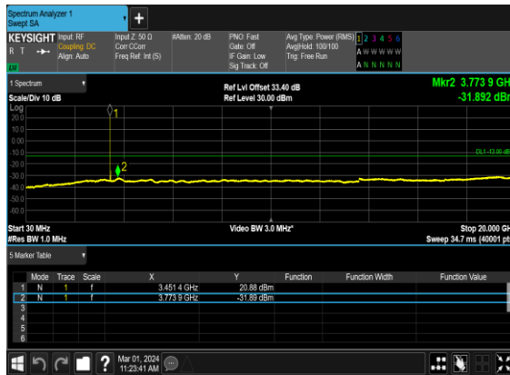
B5_N78(70M)_DFT-s-OFDM_QPSK_Edge_1RB_Left_Low_CH
