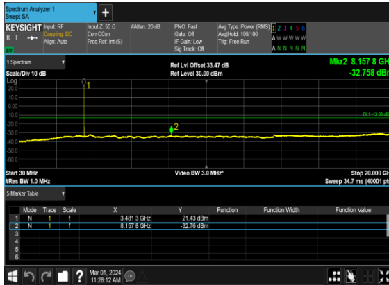
B5_N78(70M)_DFT-s- OFDM_BPSK_Edge_1RB_Left_High_CH
