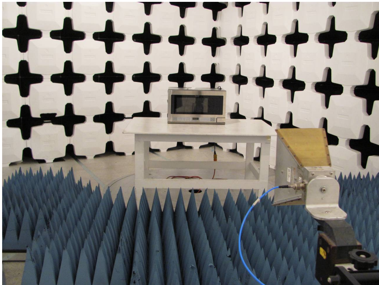
Figure 5. Radiated Emissions Measurement Photo, above 1 GHz
