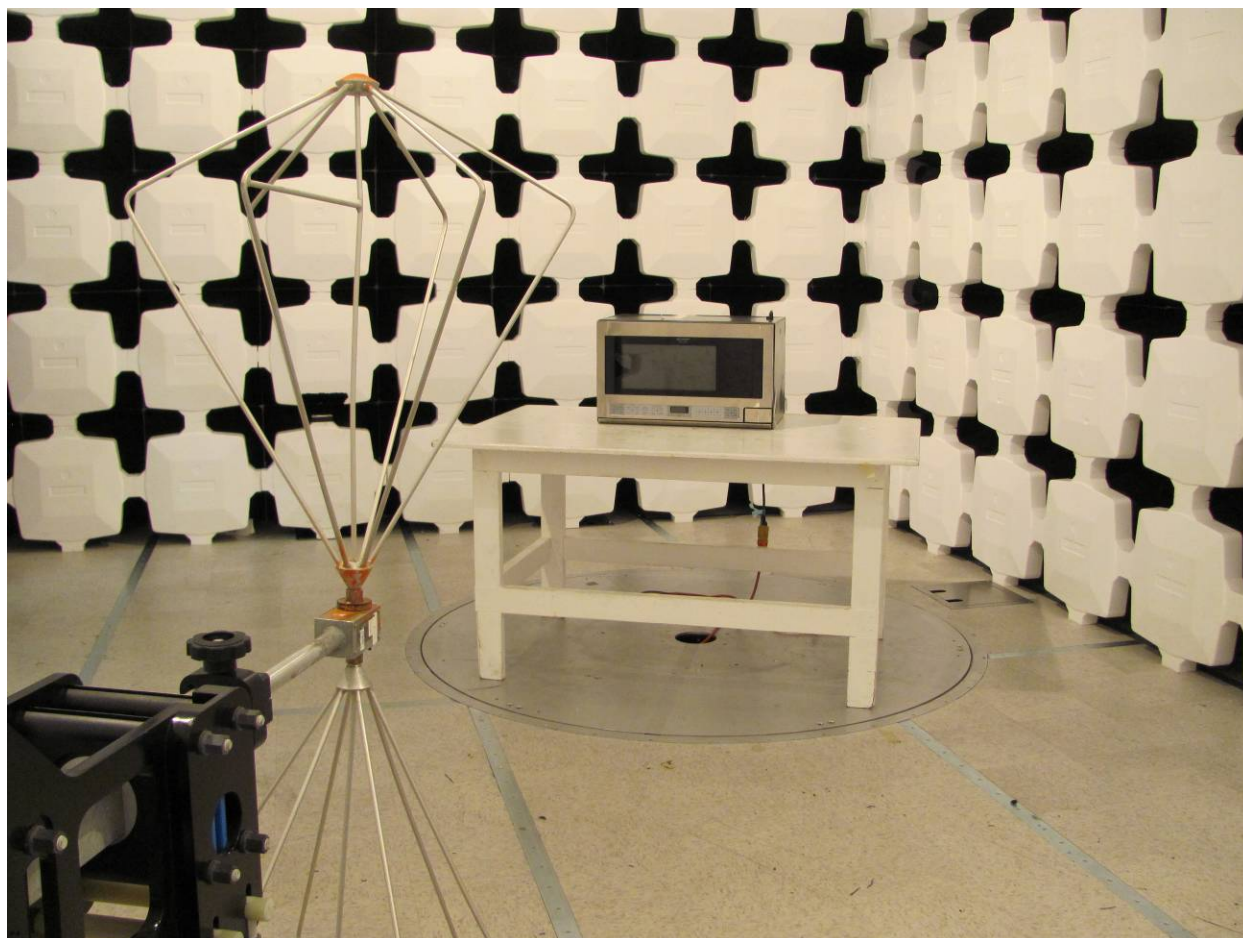
Figure 3. Radiated Emissions Measurement Photo, 30 to 200 MHz
