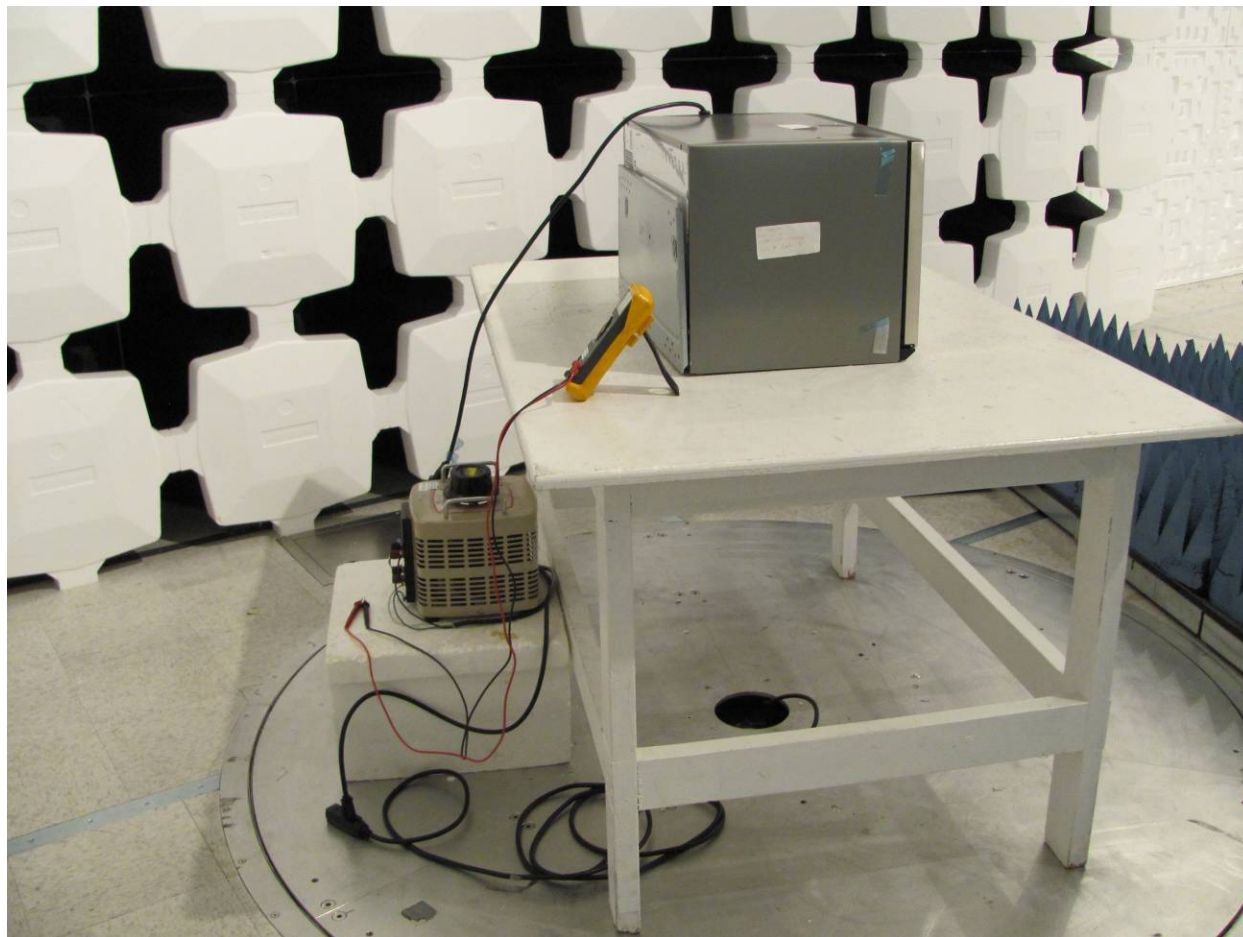
Figure 6. Frequency/Voltage Variation Test Configuration
