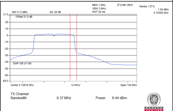
802.11ax (HE40) Beamforming / Chain 0 : CH 142 (U-NII-3)
