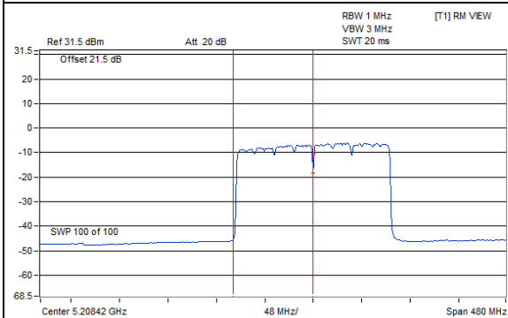
802.11ax (HE160) Beamforming / Chain 0 : CH 50 (U-NII-1)
