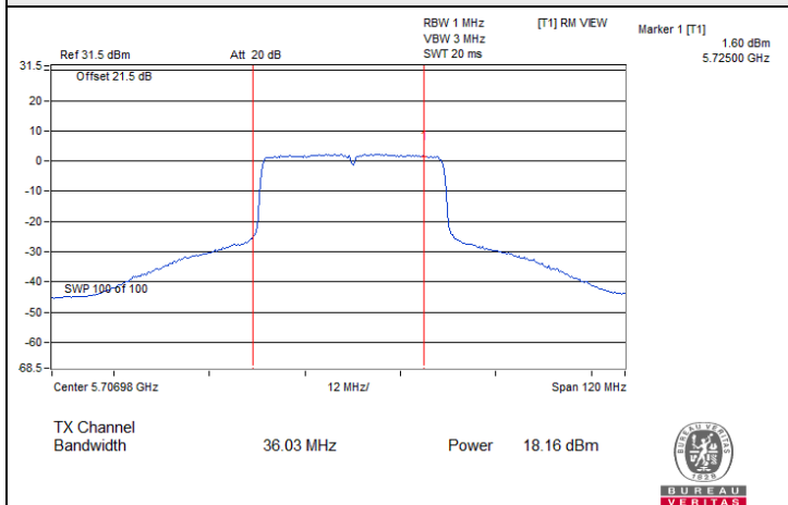
802.11ax (HE40) Beamforming / Chain 0 : CH 142 (U-NII-2C)
