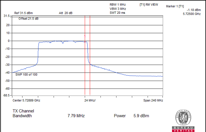
802.11ax (HE80) Beamforming / Chain 0 : CH 138 (U-NII-3)
