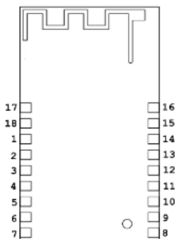
Fig 1 - pin sequence
