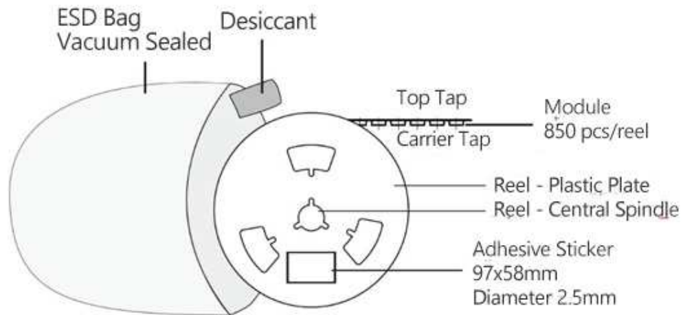
Fig 7 Packaging
