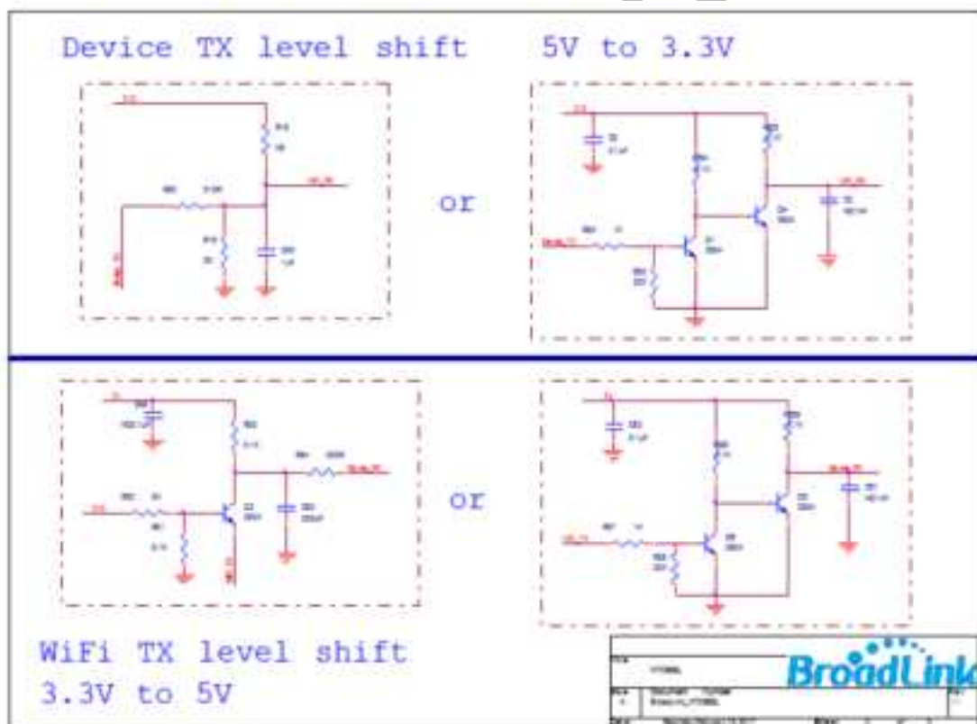
Fig 10 - Circuit Diagram (5V)
