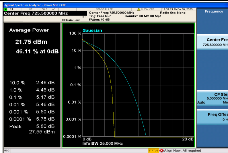
Band28-15MHz-QPSK-27435-75RB#0
