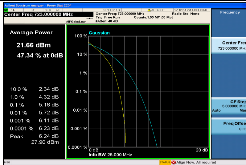
Band28-10MHz-QPSK-27410-50RB#0
