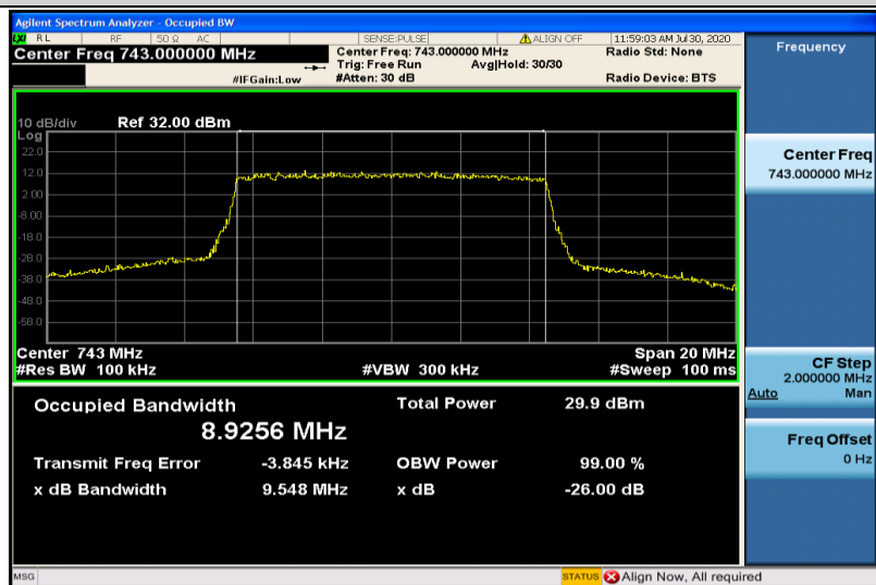
Band28-10MHz-16QAM-27610-50RB#0-8.9256
