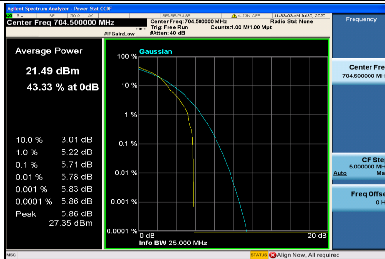
Band28-3MHz-16QAM-27225-1RB#0
