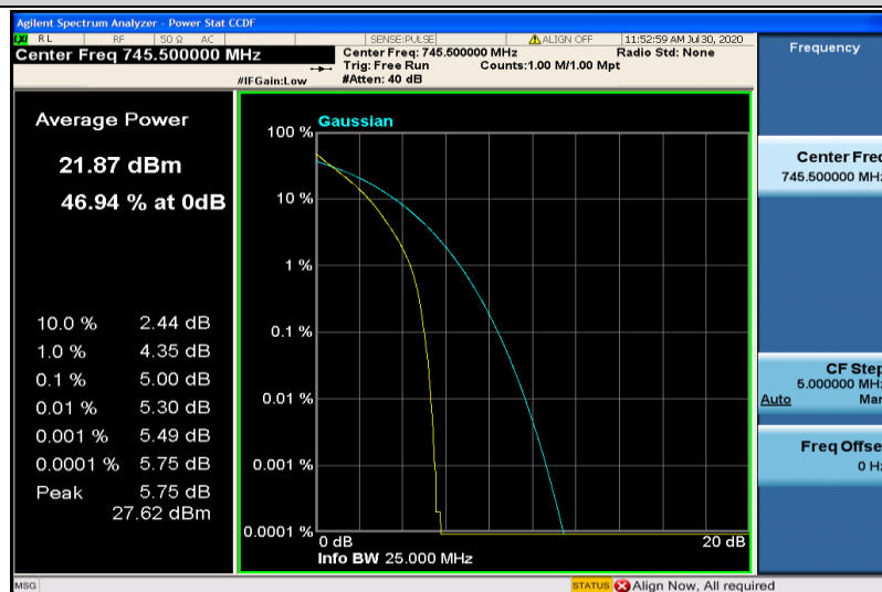
Band28-5MHz-QPSK-27635-25RB#0
