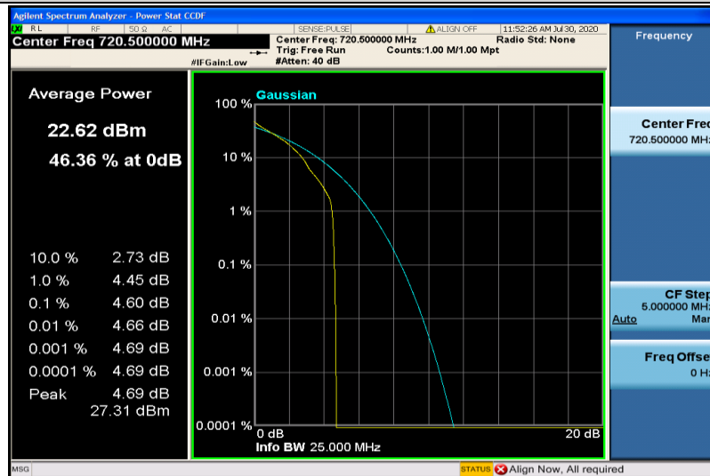
Band28-5MHz-QPSK-27385-1RB#0
