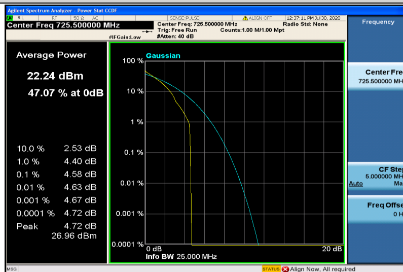
Band28-15MHz-QPSK-27435-1RB#0
