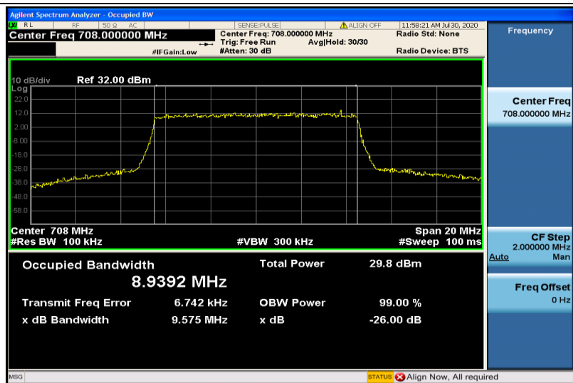
Band28-10MHz-16QAM-27260-50RB#0-8.9392
