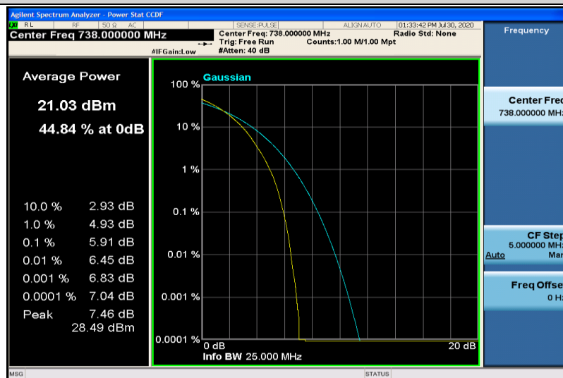
Band28-20MHz-16QAM-27560-100RB#0
