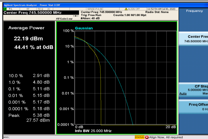
Band28-5MHz-16QAM-27635-1RB#0
