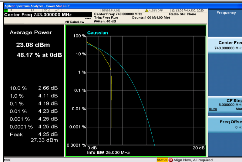
Band28-10MHz-QPSK-27610-1RB#0
