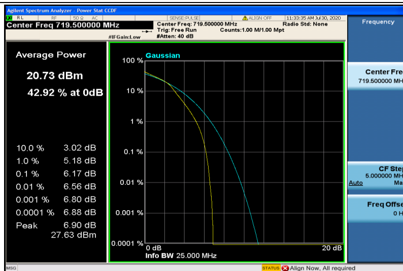
Band28-3MHz-16QAM-27375-15RB#0
