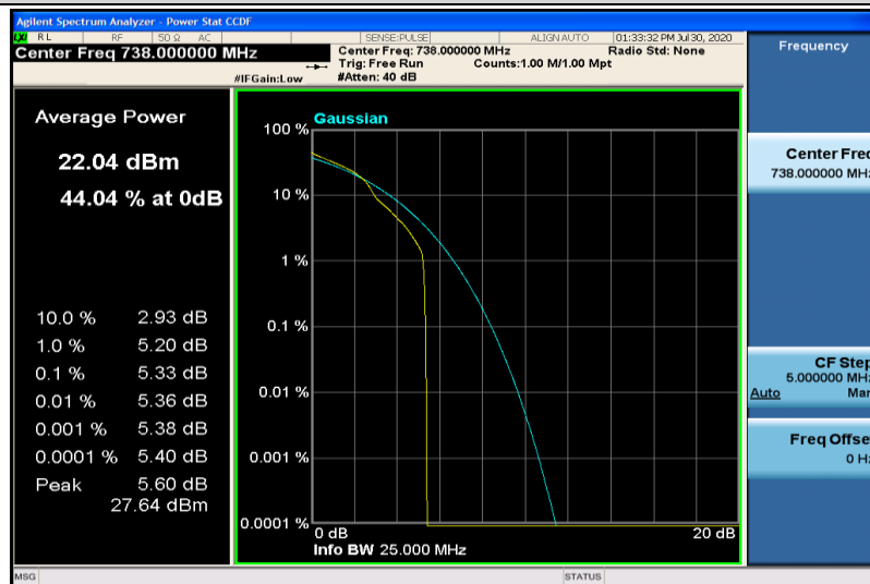
Band28-20MHz-16QAM-27560-1RB#0
