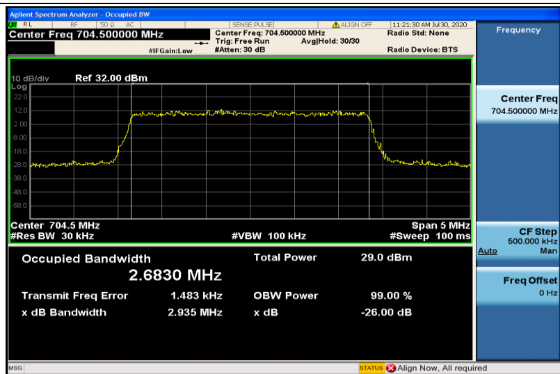
Band28-3MHz-16QAM-27225-15RB#0-2.6830
