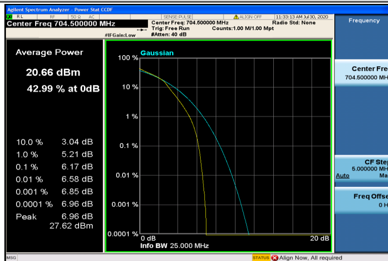
Band28-3MHz-16QAM-27225-15RB#0
