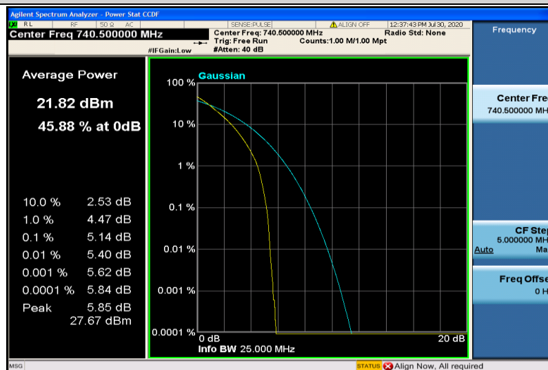
Band28-15MHz-QPSK-27585-75RB#0
