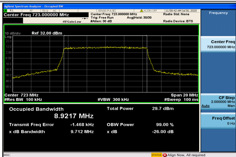
Band28-10MHz-16QAM-27410-50RB#0-8.9217
