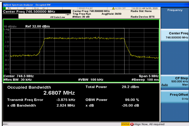
Band28-3MHz-16QAM-27645-15RB#0-2.6807
