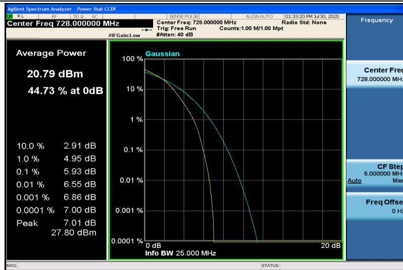
Band28-20MHz-16QAM-27460-100RB#0
