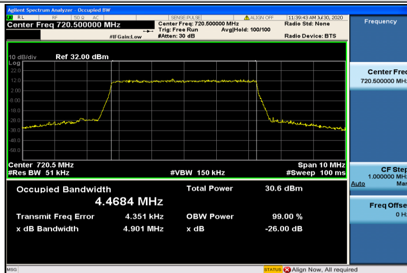
Band28-5MHz-QPSK-27385-25RB#0-4.4684
