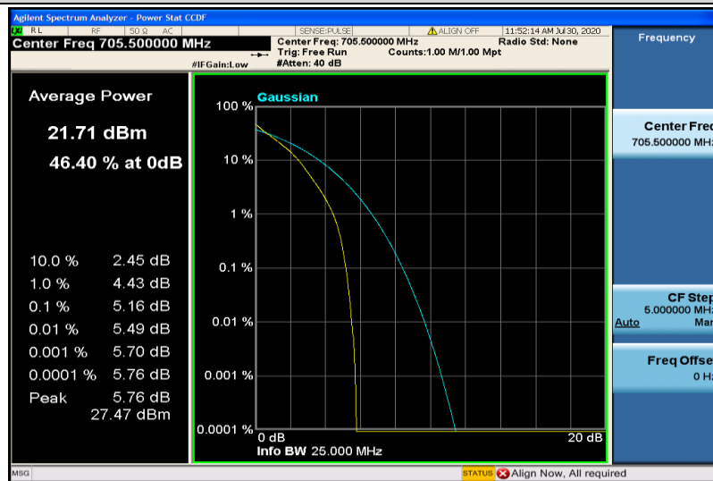
Band28-5MHz-QPSK-27235-25RB#0
