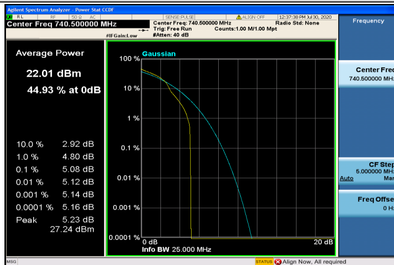
Band28-15MHz-16QAM-27585-1RB#0
