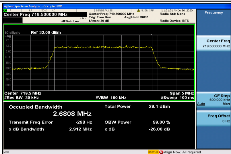
Band28-3MHz-16QAM-27375-15RB#0-2.6808
