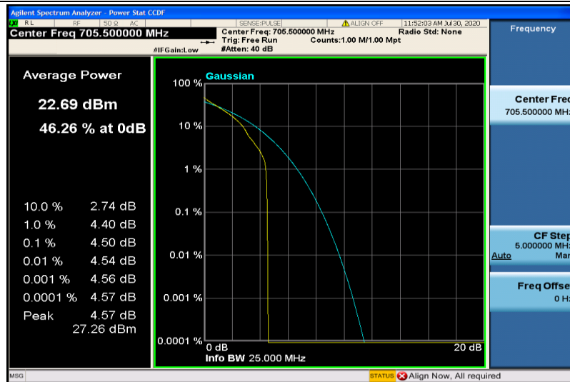
Band28-5MHz-QPSK-27235-1RB#0
