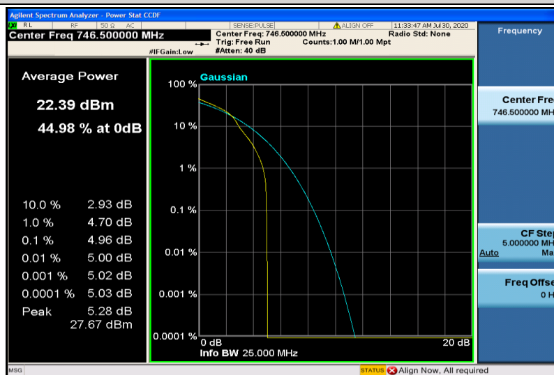
Band28-3MHz-16QAM-27645-1RB#0
