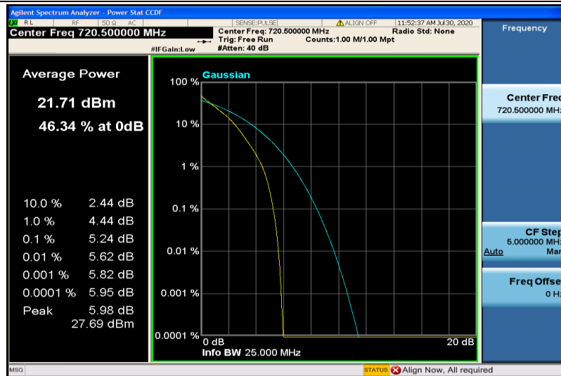
Band28-5MHz-QPSK-27385-25RB#0
