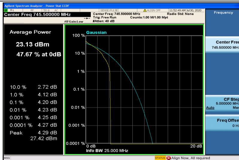
Band28-5MHz-QPSK-27635-1RB#0
