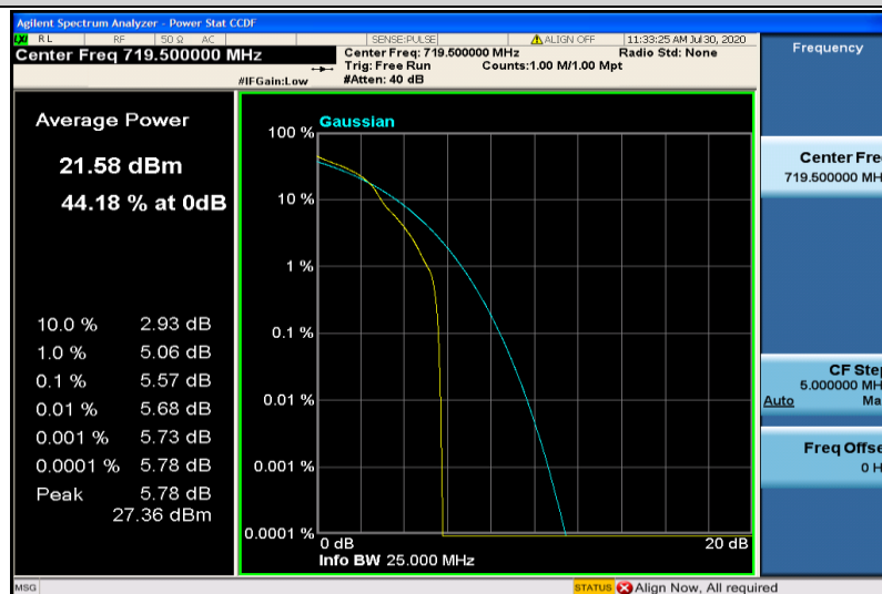
Band28-3MHz-16QAM-27375-1RB#0
