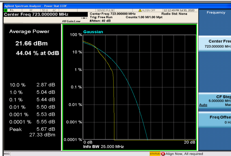
Band28-10MHz-16QAM-27410-1RB#0
