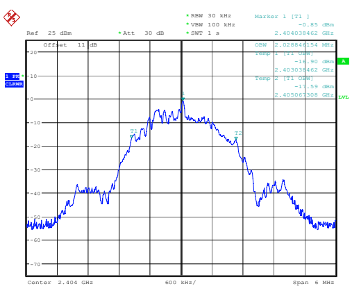
Low Channel 2.029MHz
