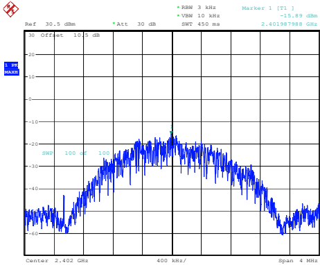
Low Channel -15.89dBm/3kHz
