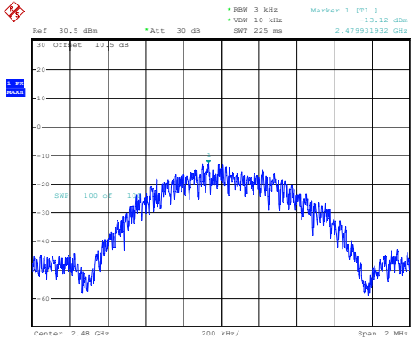
High Channel -13.12dBm/3kHz
