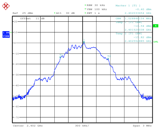
Low Channel 1.029MHz
