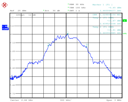
Middle Channel 1.029MHz
