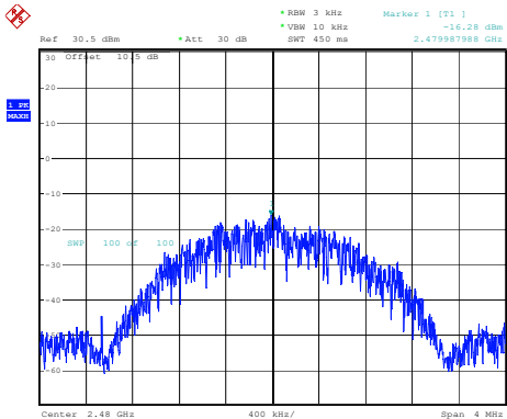
High Channel -16.28dBm/3kHz
