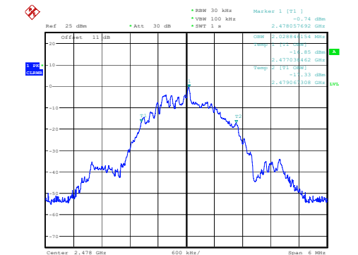
High Channel 2.029MHz
