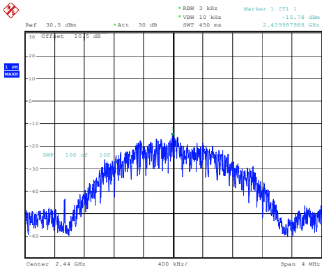
Middle Channel -15.78dBm/3kHz
