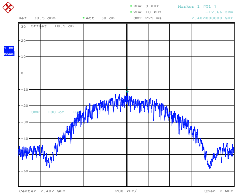
Low Channel -12.66dBm/3kHz
