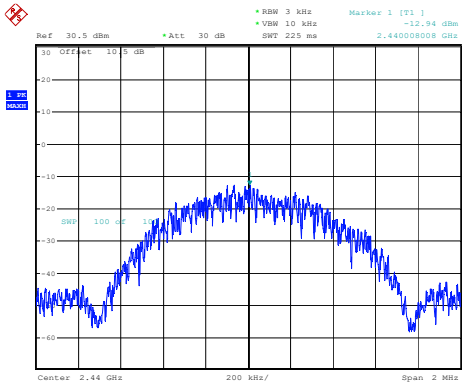
Middle Channel -12.94dBm/3kHz
