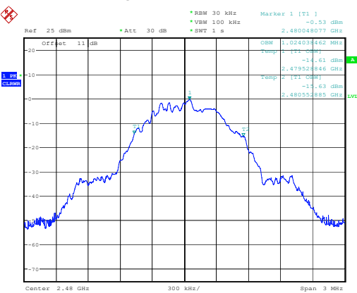
High Channel 1.024MHz
