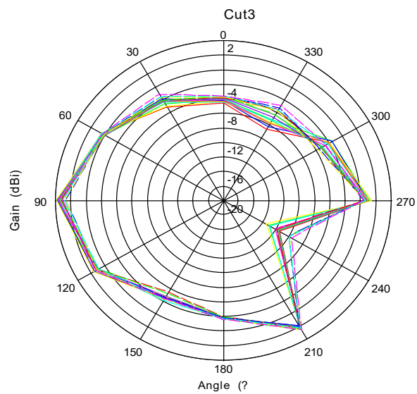
AN043 YZ Plane
