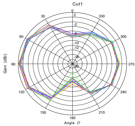
AN043 XY Plane
