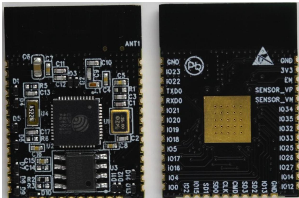
Figure 1: ESP32 Module
