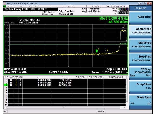
11N40SISO-Ant1-5310-PASS
