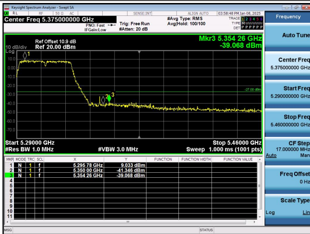
11N40SISO-Ant2-5310-PASS
