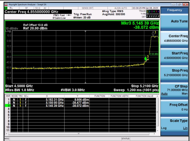
11AC40SISO-Ant2-5190-PASS
