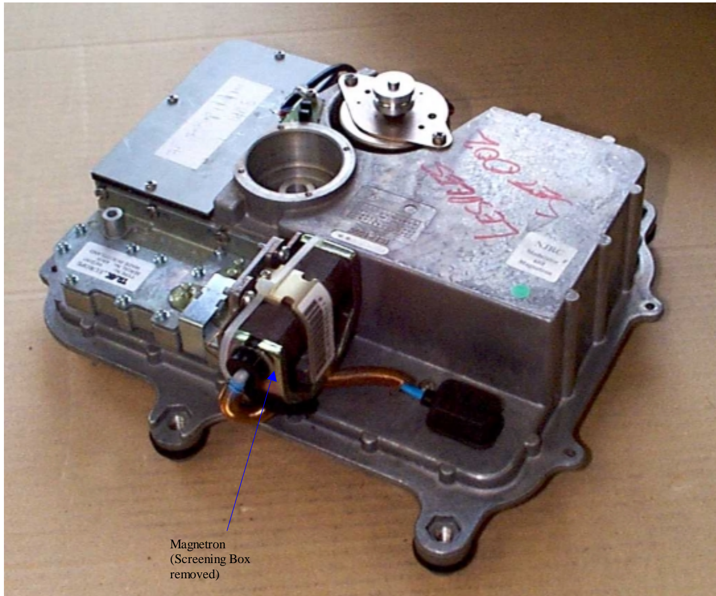
2D – 2kW (8-Pulse Width), 18" Radome Scanner Unit
