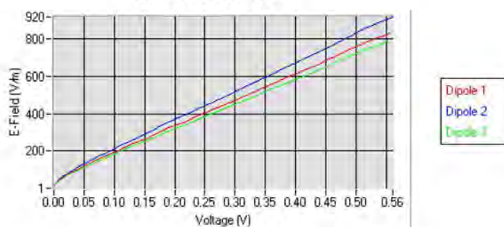
Calibration curves
