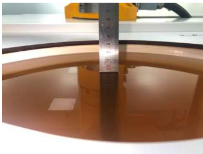
Fig. 9.2 Photo of Liquid Height for Body SAR (1700MHz~2000MHz) (depth>15cm)
