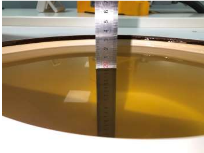
Fig. 9.3 Photo of Liquid Height for Body SAR (2000MHz~2600MHz) (depth>15cm)
