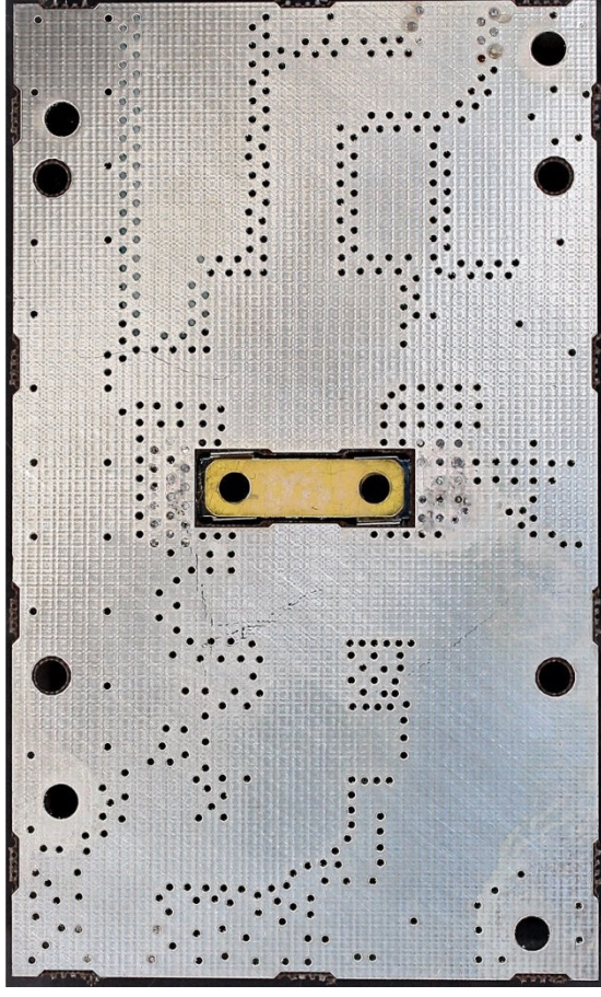
Photograph 17: Power Amplifier 60W PA 2 PCB – Top & Bottom
