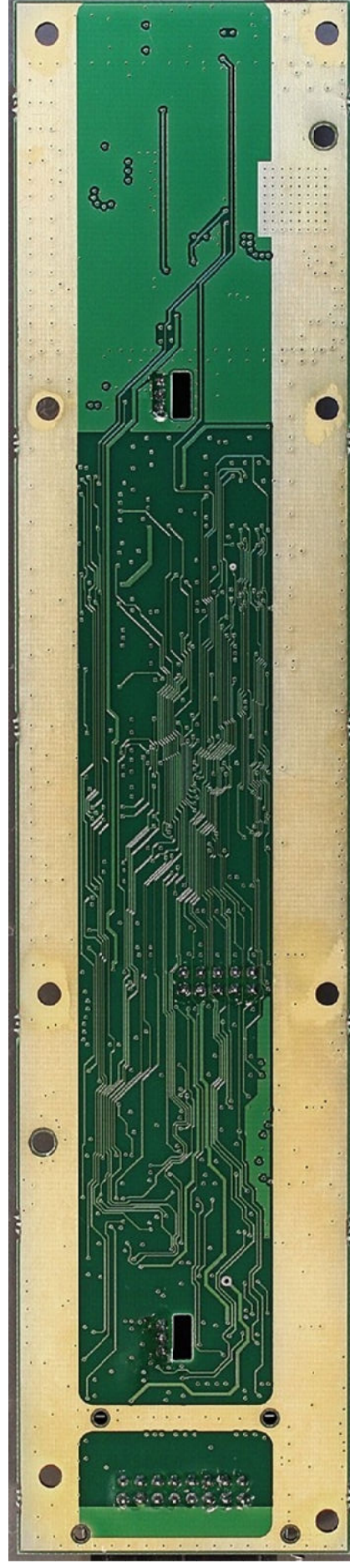
Photograph 21: Power Amplifier Control PCB – Top & Bottom
