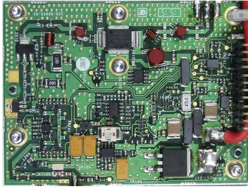
Photograph 14: Power Amplifier 6W Driver PCB – Top & Bottom
