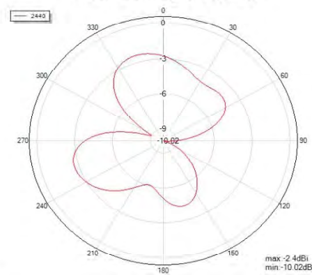
Theta=90 freq=2440MHz
