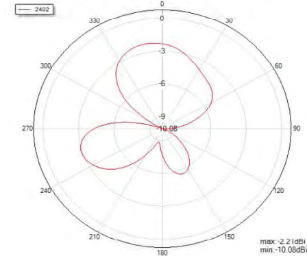
Theta=90 freq=2402MHz
