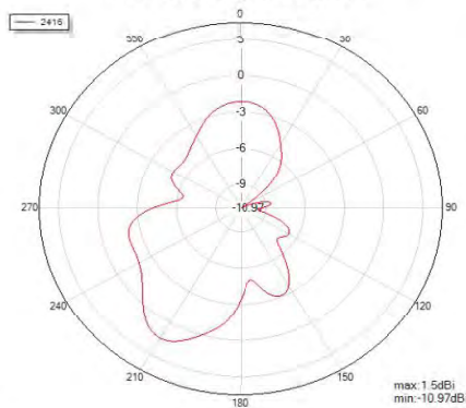
Phi=90 freq=2416MHz
