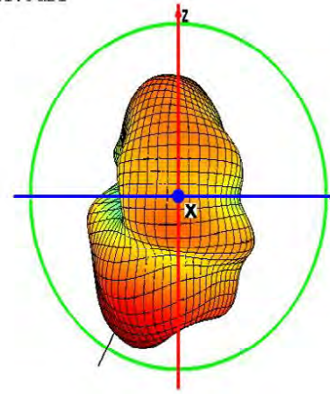
Theta=90 freq=2402MHz
