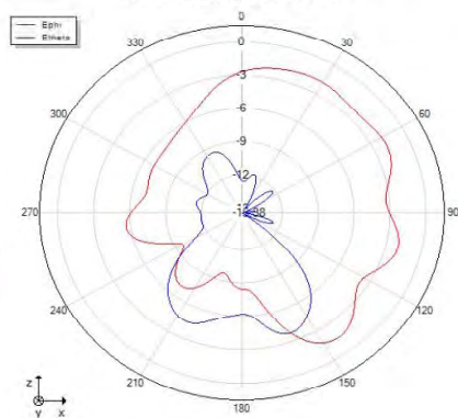
Phi=0 freq=2440MHz
