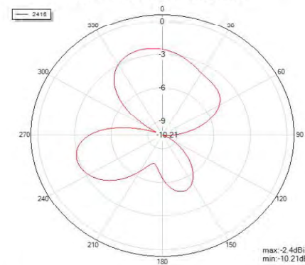
Theta=90 freq=2416MHz
