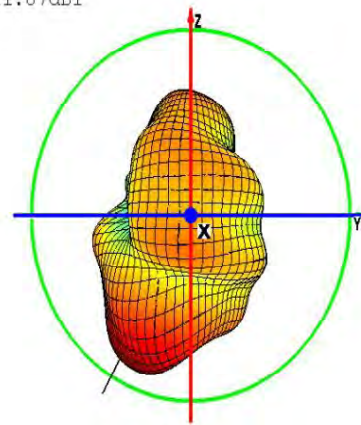
Theta=90 freq=2416MHz
