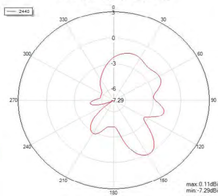
Phi=0 freq=2440MHz
