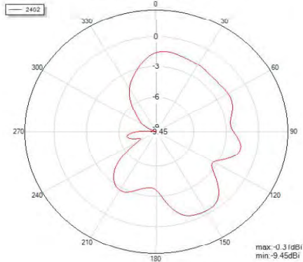
Phi=0 freq=2402MHz
