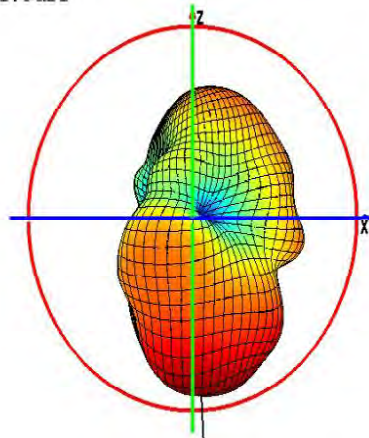
Phi=0 freq=2402MHz
