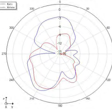
Phi=90 freq=2402MHz
