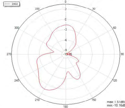
Phi=90 freq=2402MHz
