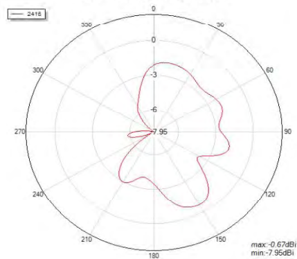
Phi=0 freq=2416MHz
