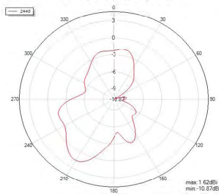
Phi=90 freq=2440MHz
