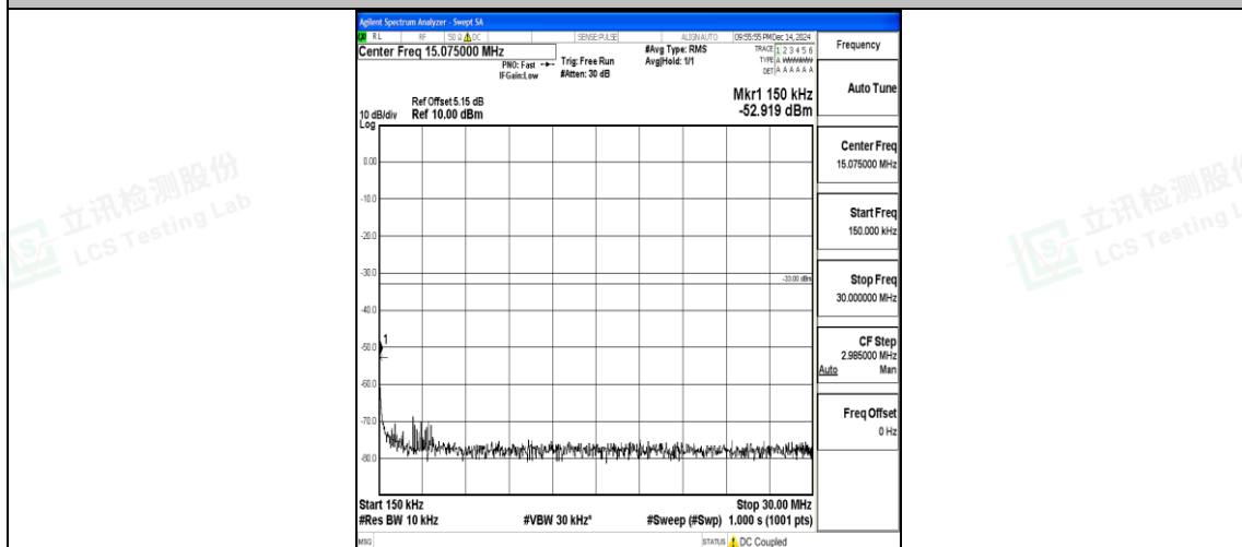
Band25_1.4MHz_16QAM_26683_1RB#0_0.15~30_0.15~30
