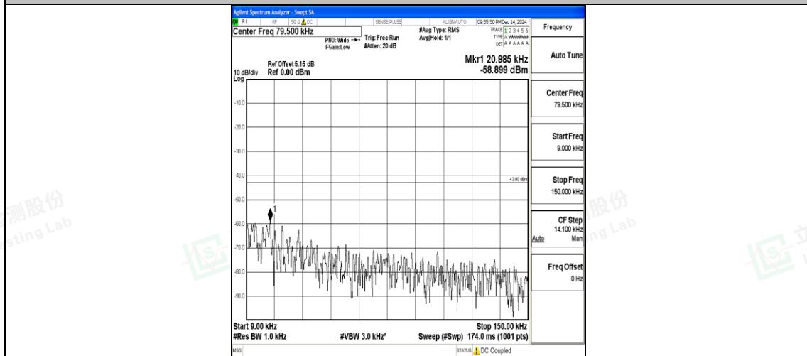
Band25_1.4MHz_16QAM_26683_1RB#0_0.009~0.15_0.009~0.15
