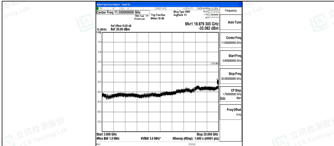
Band25_1.4MHz_QPSK_26683_1RB#0_3000~20000_3000~20000
