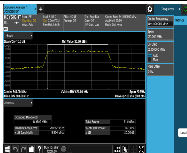
Band5-10MHz-16QAM-20600-50RB#0
