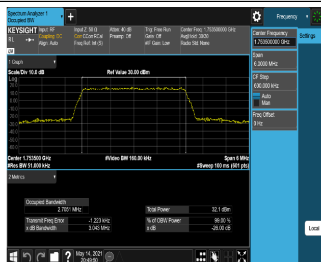
Band4-3MHz-16QAM-20385-15RB#0
