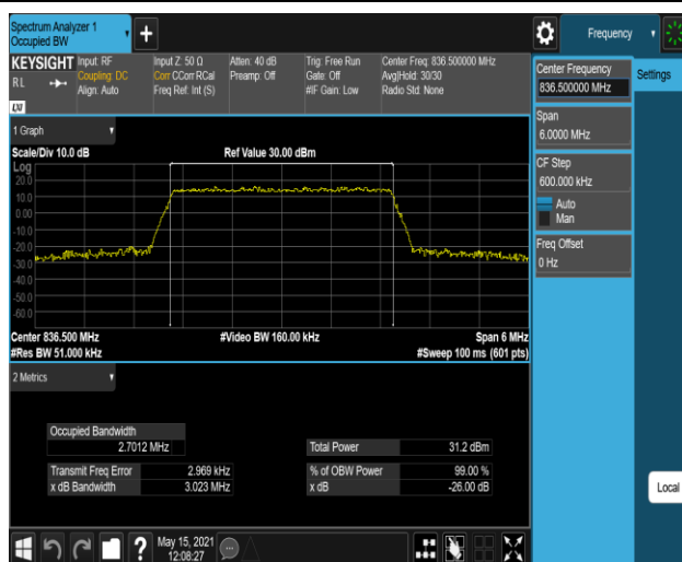
Band5-3MHz-16QAM-20525-15RB#0
