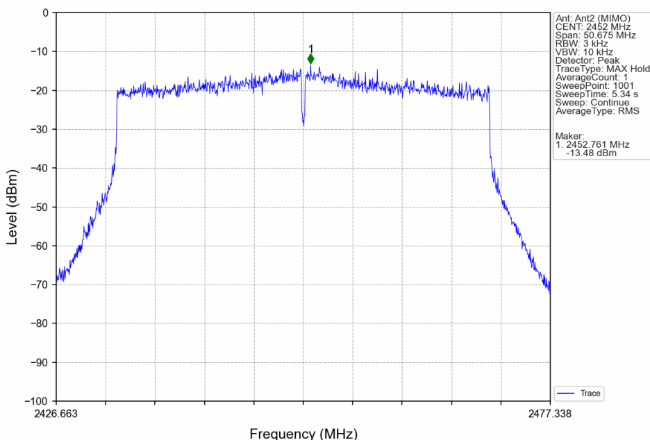
802.11ax(HEW40)_HCH_2452MHz_RU484_Left_MIMO_NTNV
