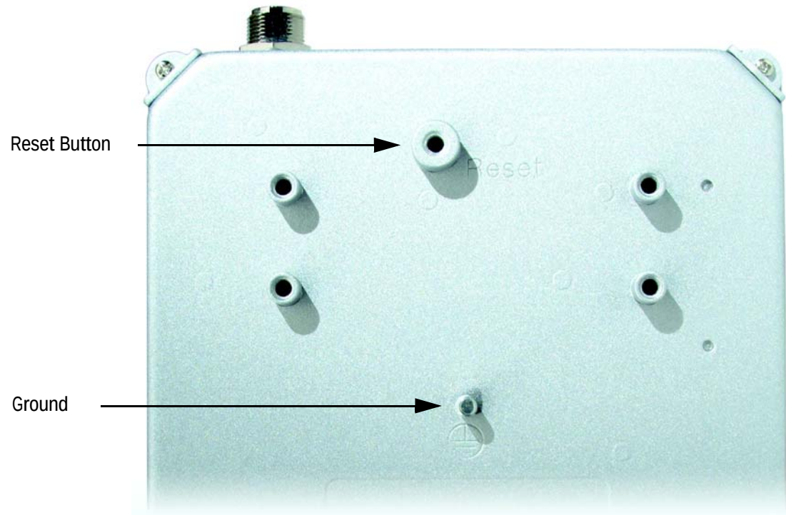
Figure 3-4: Reset Button
