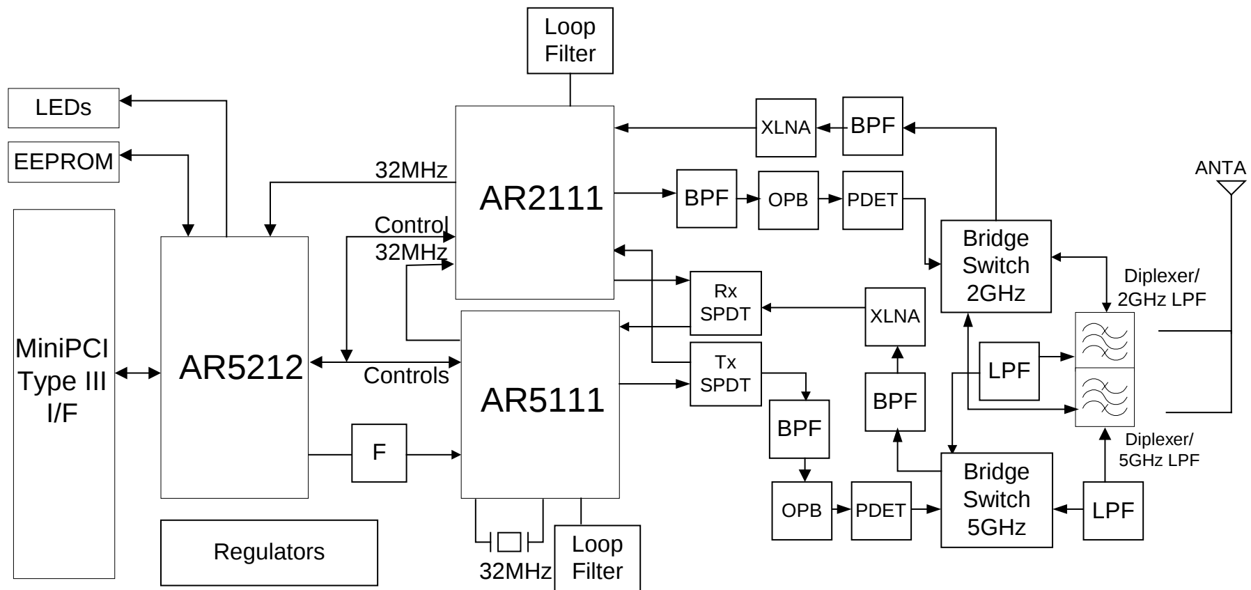
T60H677T05 Block Diagram ( Operation frequency:2.4~2.5GHz & 5.15~5.85GHz )
