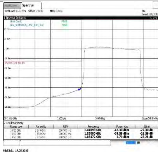
Band25-20MHz-16QAM-26140-100RB#0
