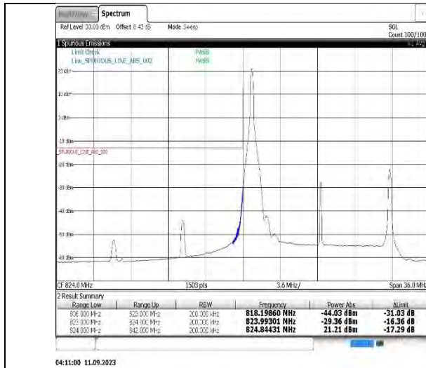
Band26(824-849)-15MHz-QPSK-26965-1RB#74
