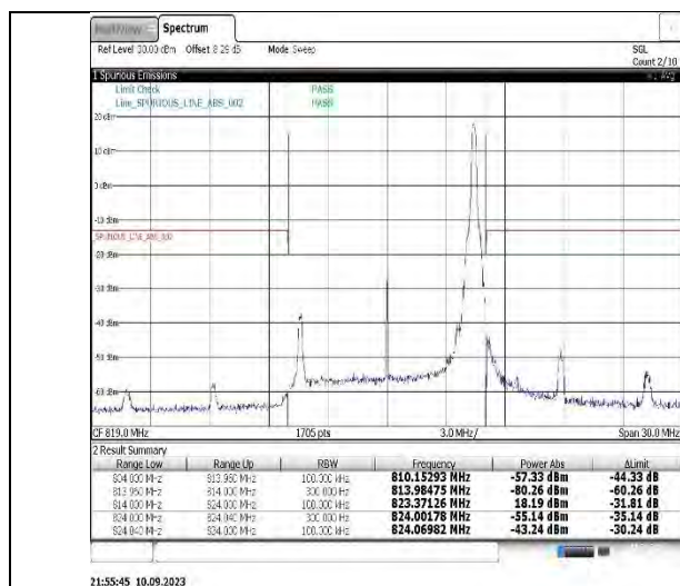
Band26(824-849)-10MHz-16QAM-26840-1RB#0
