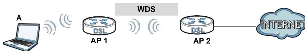
Figure 42 WDS Link Example
