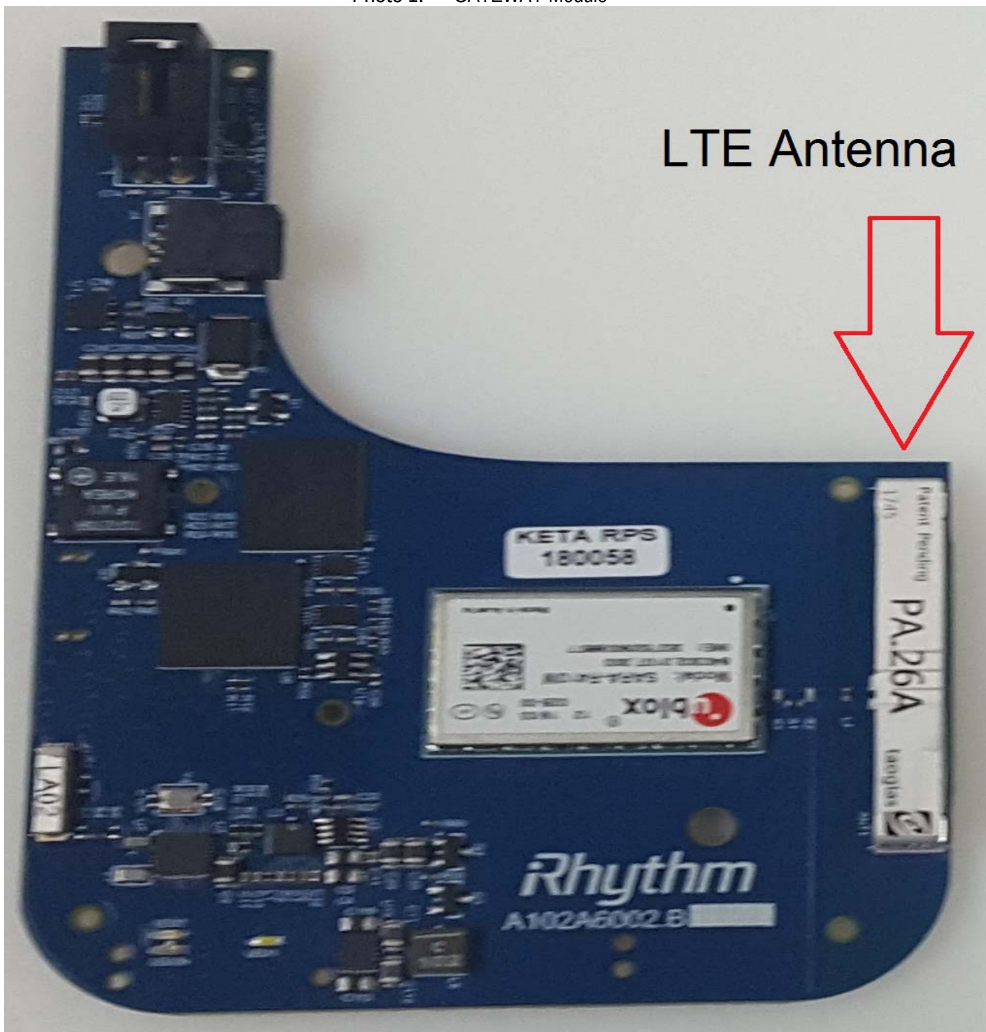
Photo 1: GATEWAY Module
