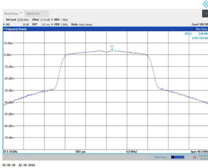
11A_Ant3_5180
