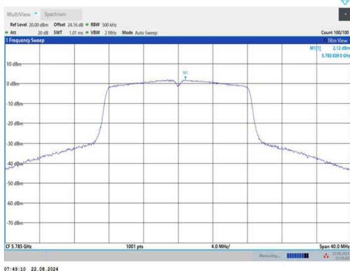
11A_Ant3_5785
