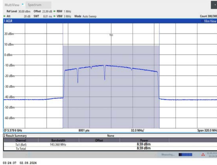
11BE160MIMO_Ant1_5570_996+484+242_OFDMA_1
