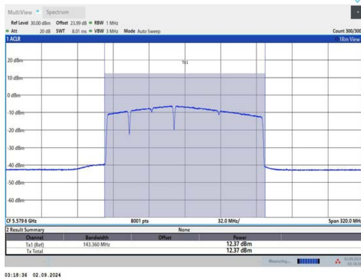
11BE160MIMO_Ant1_5570_996+484+242_OFDMA_2
