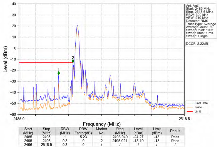
Band41_15MHz_16QAM_LCH_2503.5MHz_RB_1_0_NTNV
