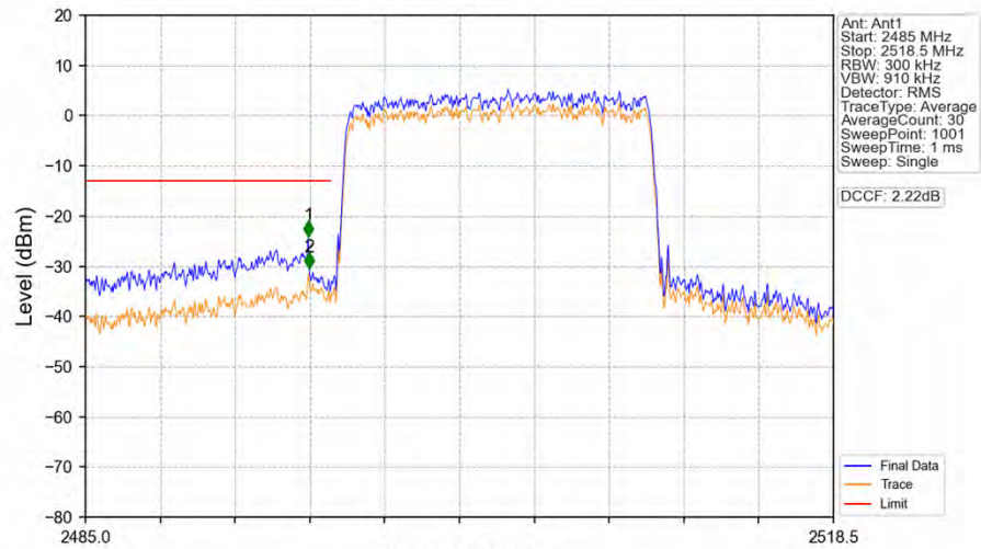
Band41_15MHz_16QAM_LCH_2503.5MHz_RB_75_0_NTNV
