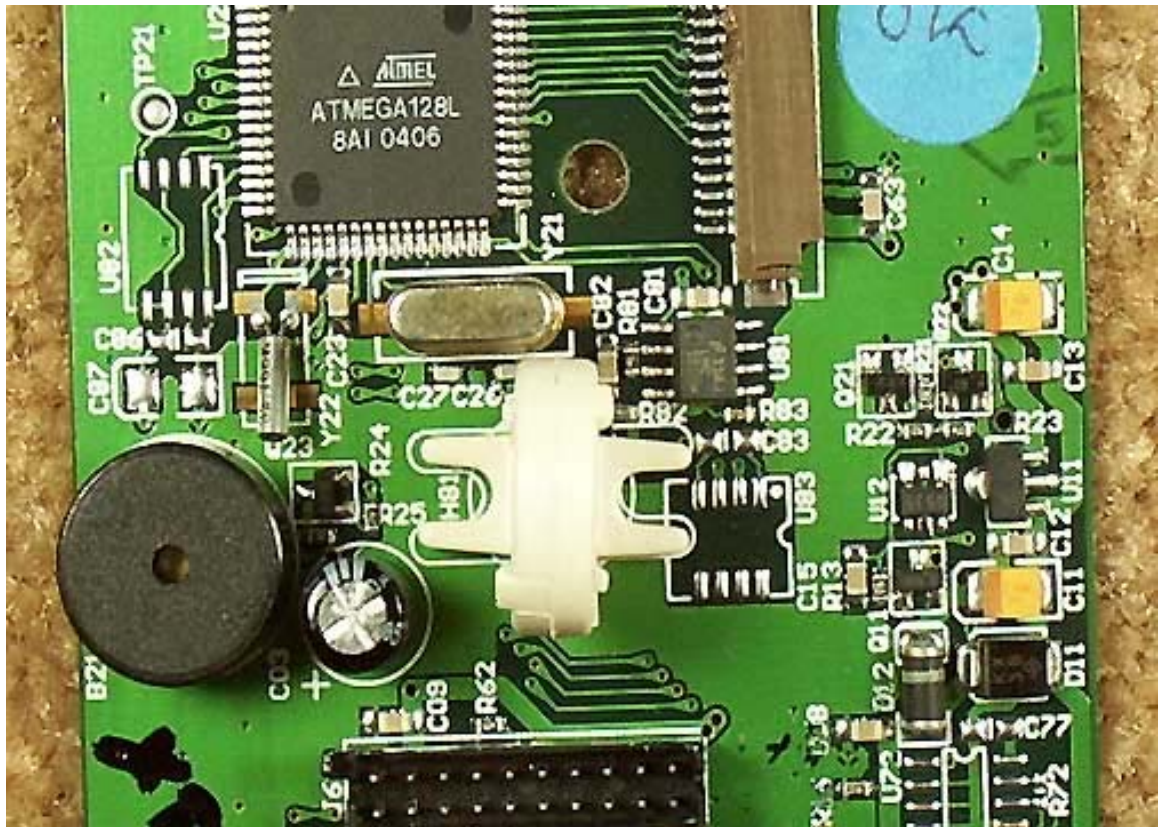
PCB Front 2
