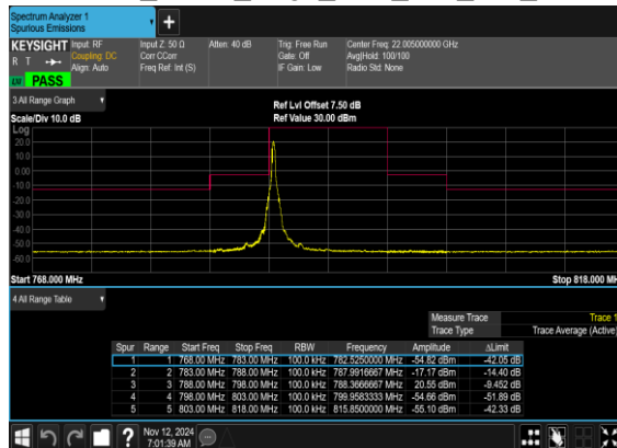
N14(10M)_DFT-s- OFDM_BPSK_Edge_1RB_Left_Mid_CH
