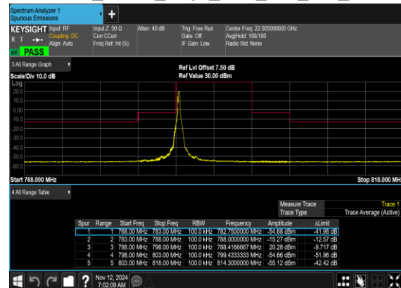
N14(10M)_DFT-s- OFDM_QPSK_Edge_1RB_Left_Mid_CH
