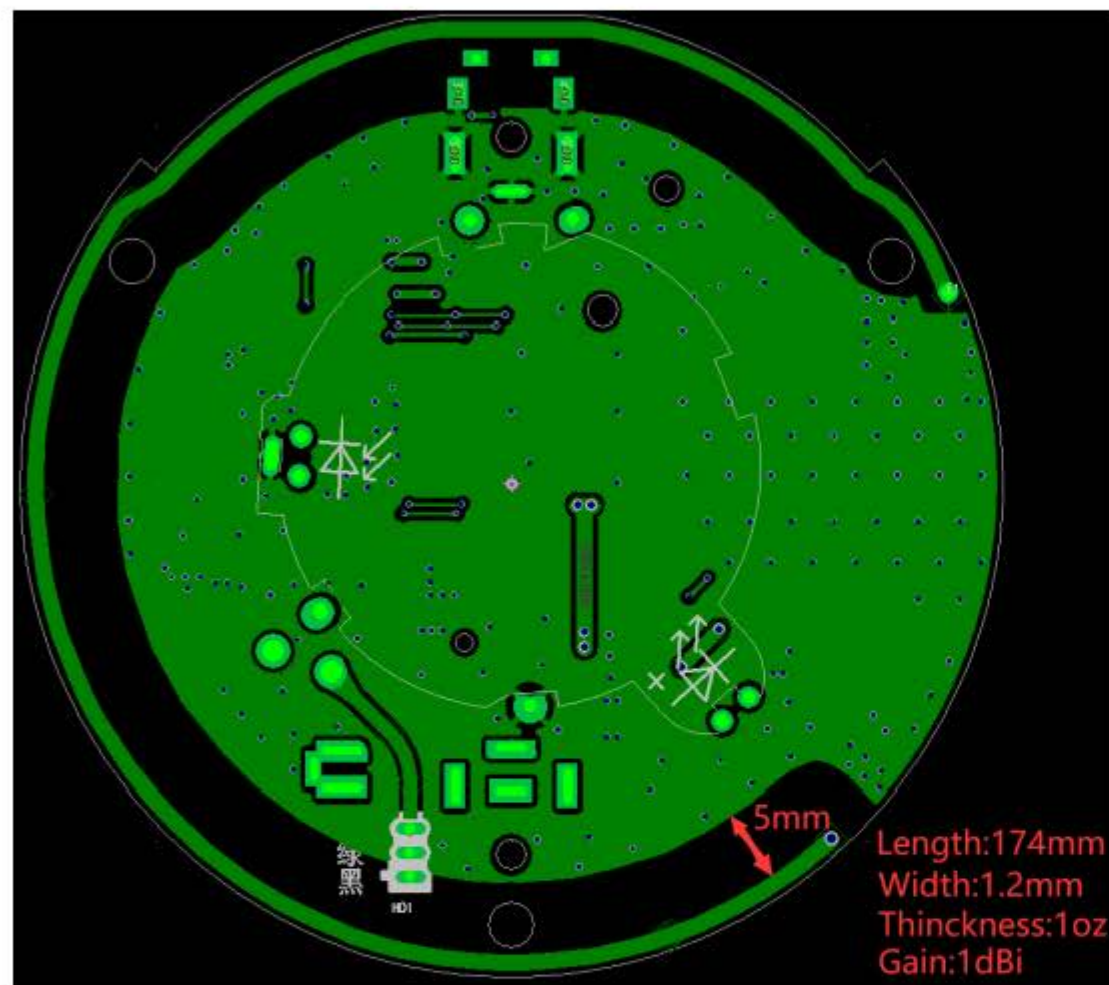
PCB Design Drawing
