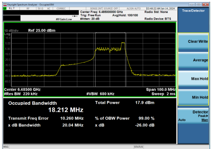
Plot 7-23. 26dB & 99% Bandwidth Plot Antenna WF5B (40MHz 802.11ax RU26 (UNII Band 6) - Ch. 107)
