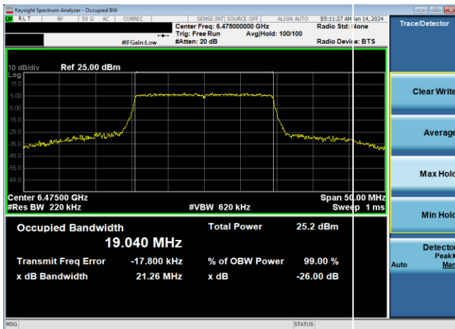
Plot 7-20. 26dB & 99% Bandwidth Plot Antenna WF5B (20MHz 802.11ax RU242 (UNII Band 6) - Ch. 105)
