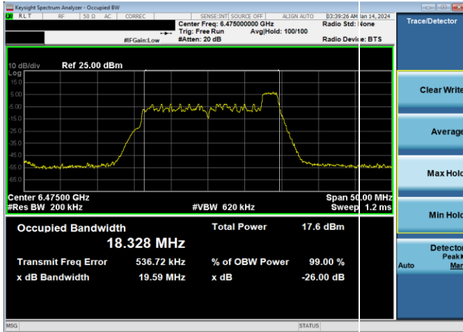
Plot 7-19. 26dB & 99% Bandwidth Plot Antenna WF5B (20MHz 802.11ax RU26 (UNII Band 6) - Ch. 105)
