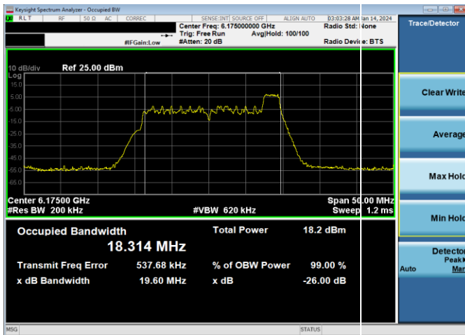
Plot 7-3. 26dB & 99% Bandwidth Plot Antenna WF5B (20MHz 802.11ax RU26 (UNII Band 5) – Ch. 45)
