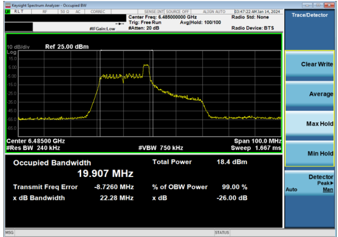
Plot 7-22. 26dB & 99% Bandwidth Plot Antenna WF5B (40MHz 802.11ax RU26 (UNII Band 6) - Ch. 107)
