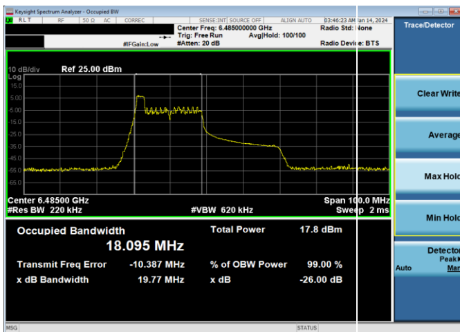
Plot 7-21. 26dB & 99% Bandwidth Plot Antenna WF5B (40MHz 802.11ax RU26 (UNII Band 6) - Ch. 107)
