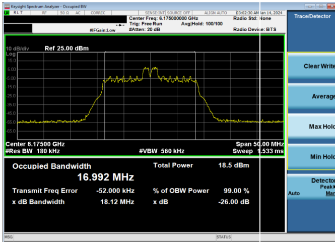
Plot 7-2. 26dB & 99% Bandwidth Plot Antenna WF5B (20MHz 802.11ax RU26 (UNII Band 5) – Ch. 45)
