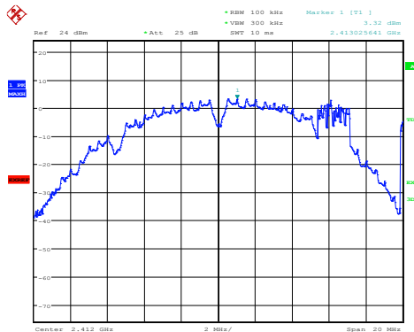
11b – 2412 MHz PSD
