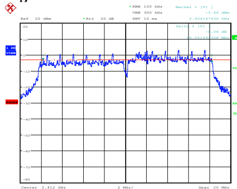
11g – 2412 MHz Bandwidth
