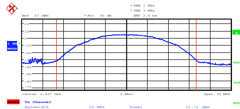
11b – 2437 MHz Power
