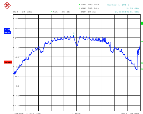
11b – 2437 MHz PSD
