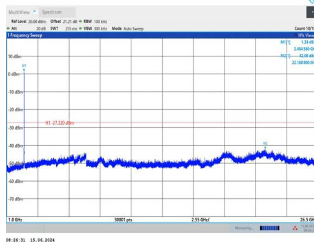
11N20SISO_Ant1_2437_0~Reference
