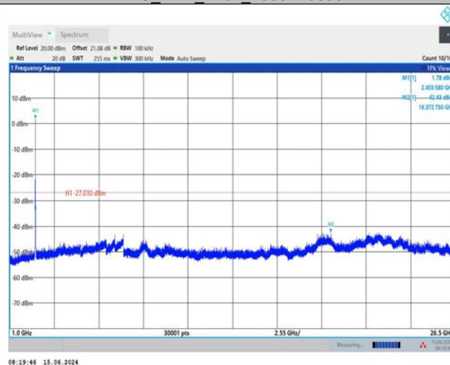
11N20SISO_Ant1_2412_0~Reference
