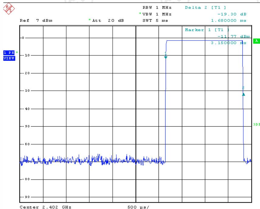
2402 MHz_DH3
