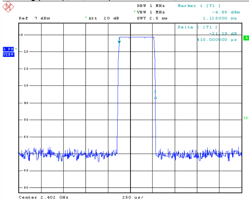
2402 MHz_DH1
