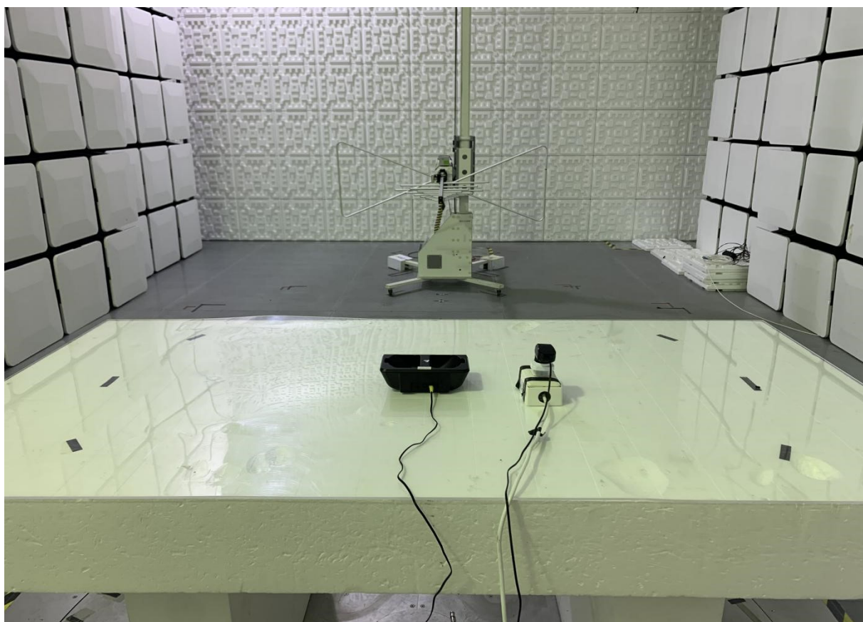
Photograph 1: Set-up photo for Radiated Spurious Emission, up to 1GHz
