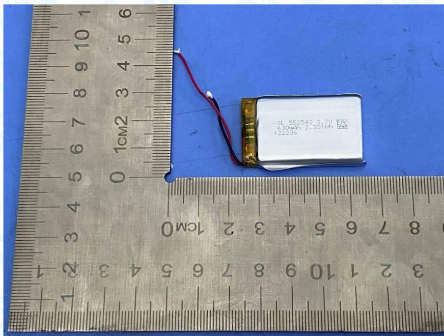
Photo 11 Internal of Battery
