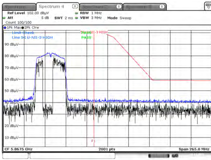
Peak Result (802.11n_HT40, Ch.159, X-V)
