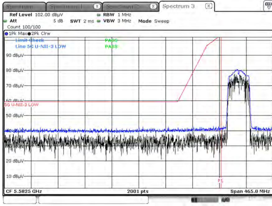
Peak Result (802.11ac_VHT40, Ch.151, X-V)
