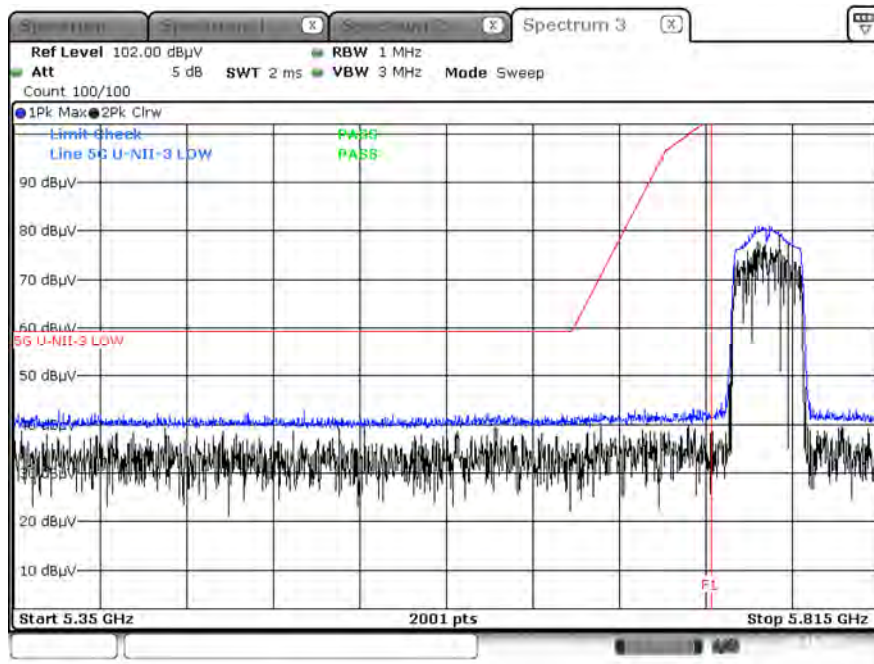
Peak Result (802.11n_HT40, Ch.151, X-V)
