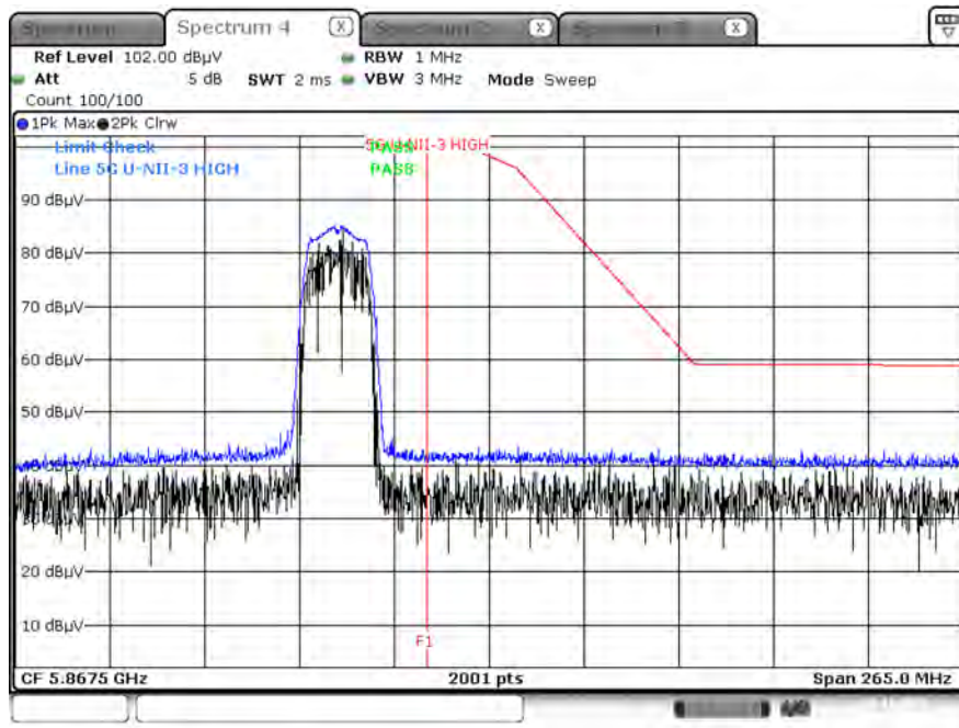
Peak Result (802.11ac_VHT20, Ch.165, X-V)
