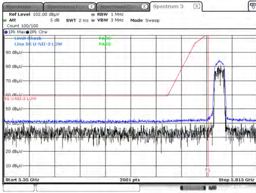
Peak Result (802.11ac_VHT20, Ch.149, X-V)
